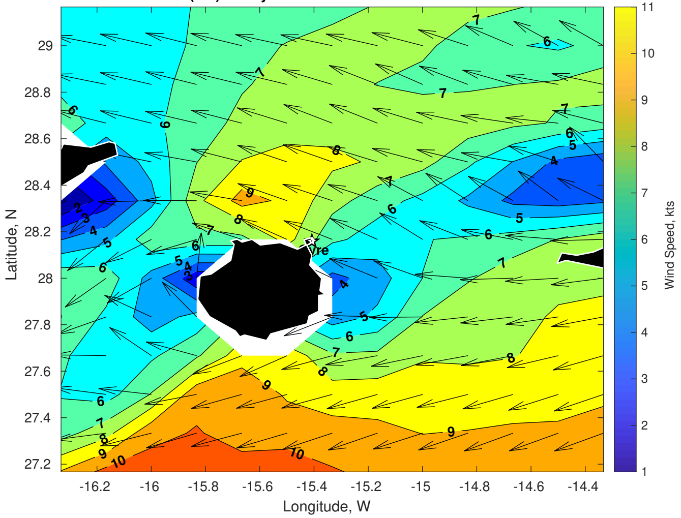
Winds (kts) for Gyre at 09-Feb-2025 09:00:00
