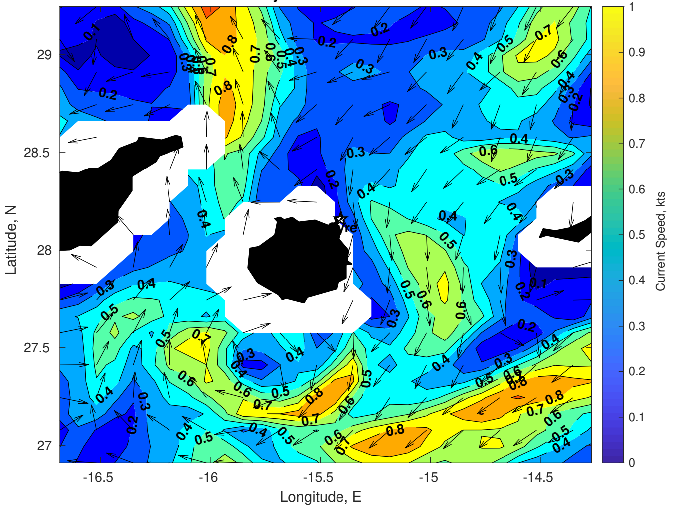
Surface Currents for Gyre at 08-Feb-2025 00:00:00
