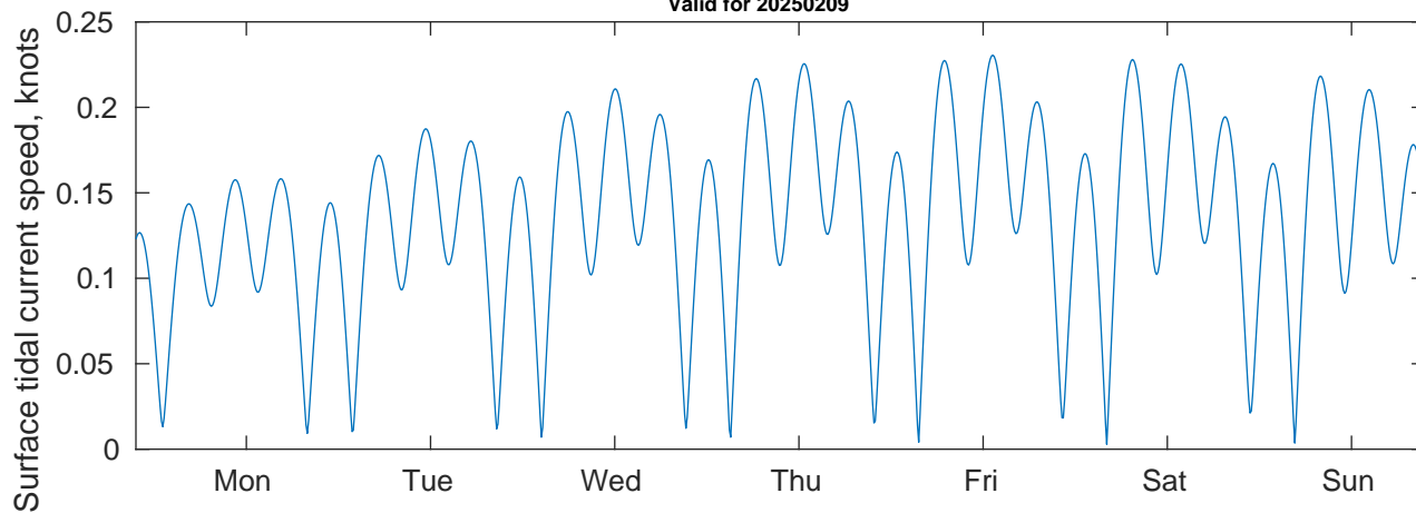
Tidal Currents and Heights for Gyre at 20250209
