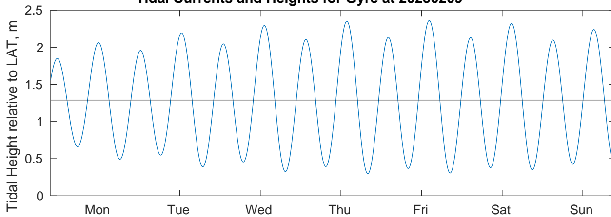
Tidal Currents and Heights for Gyre at 20250209
