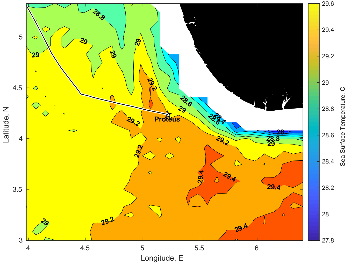
SST for Proteus at 08-Feb-2025 00:00:00
