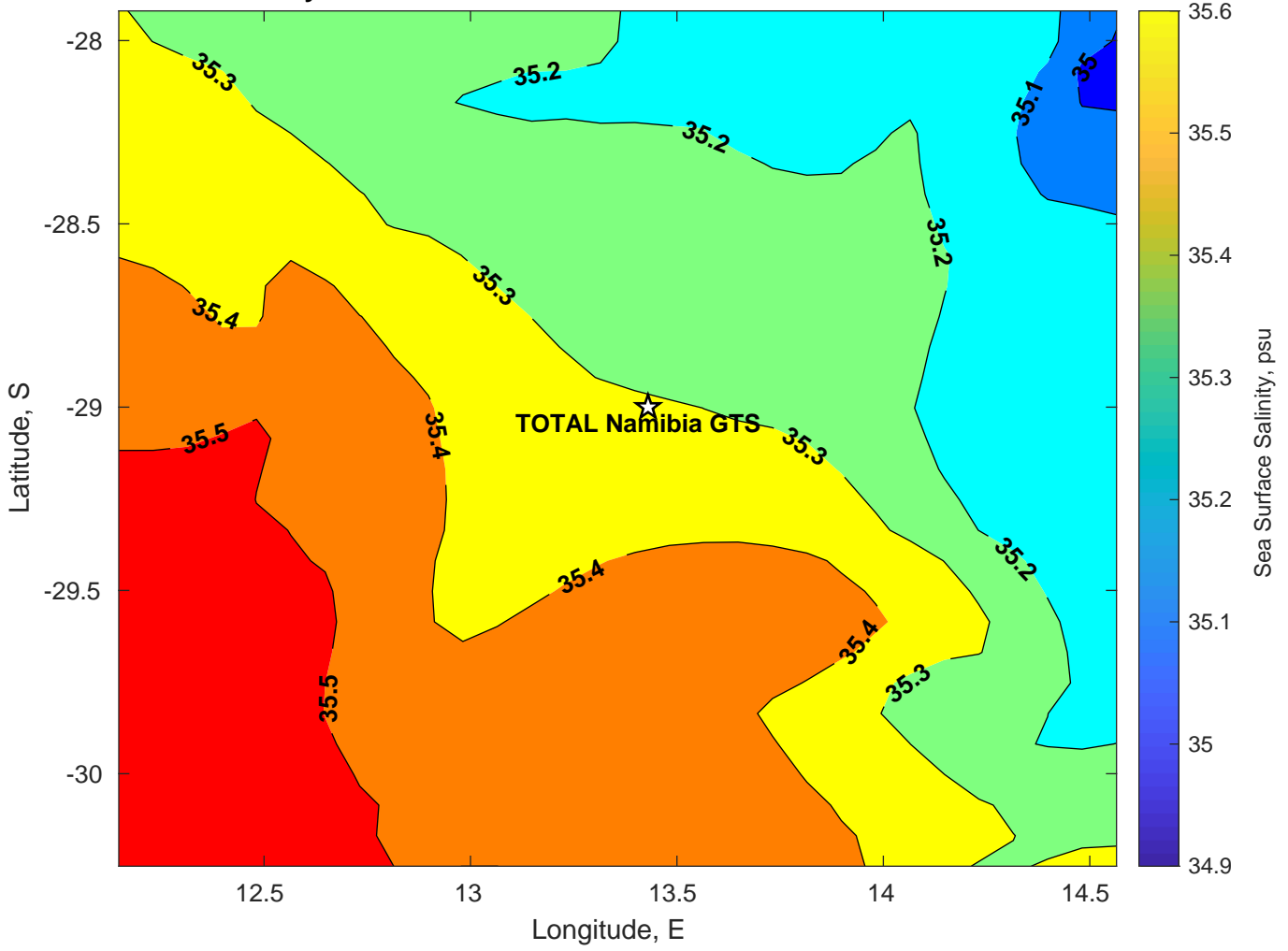
Surface Salinity for TOTAL Namibia GTS at 08-Feb-2025 00:00:00
