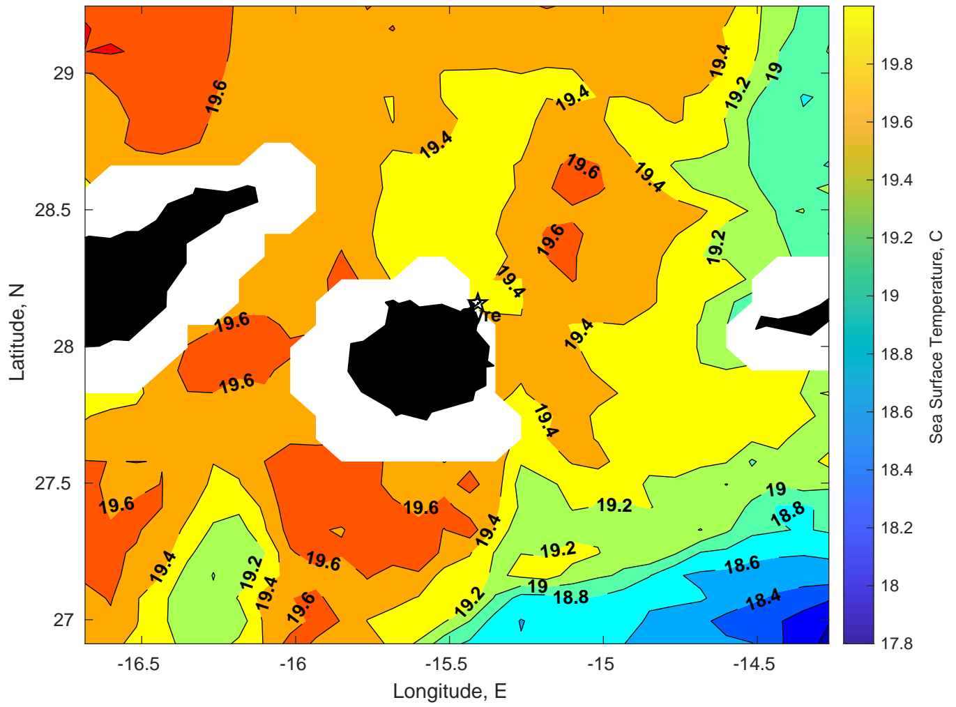
SST for Gyre at 09-Feb-2025 00:00:00
