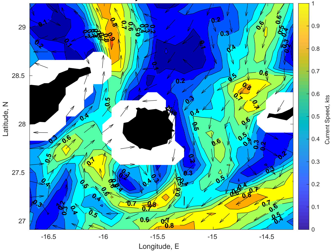
Surface Currents for Gyre at 09-Feb-2025 00:00:00
