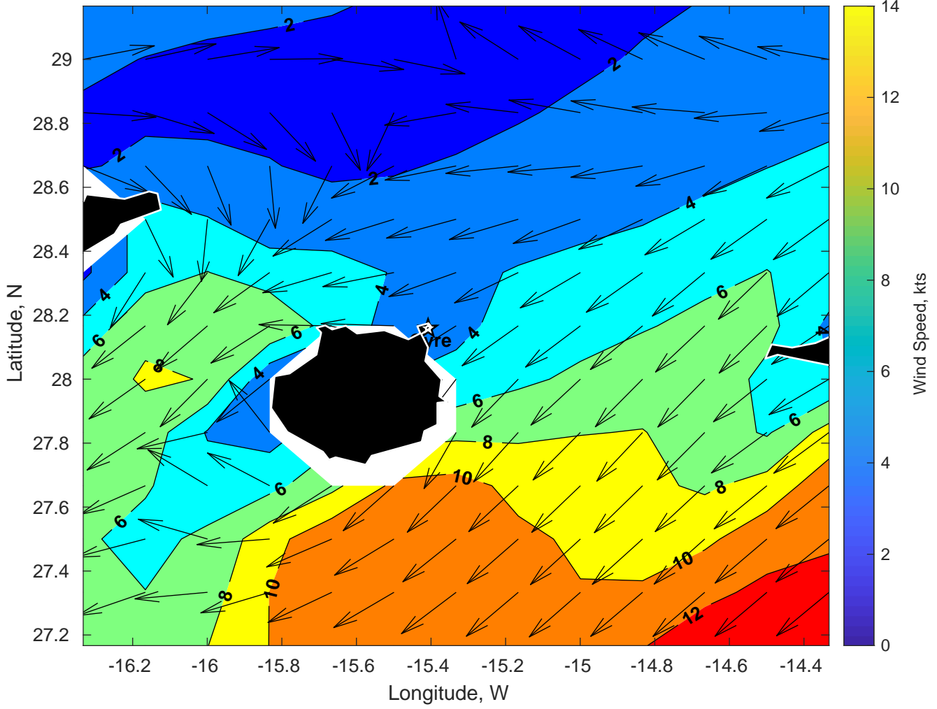
Winds (kts) for Gyre at 10-Feb-2025 09:00:00
