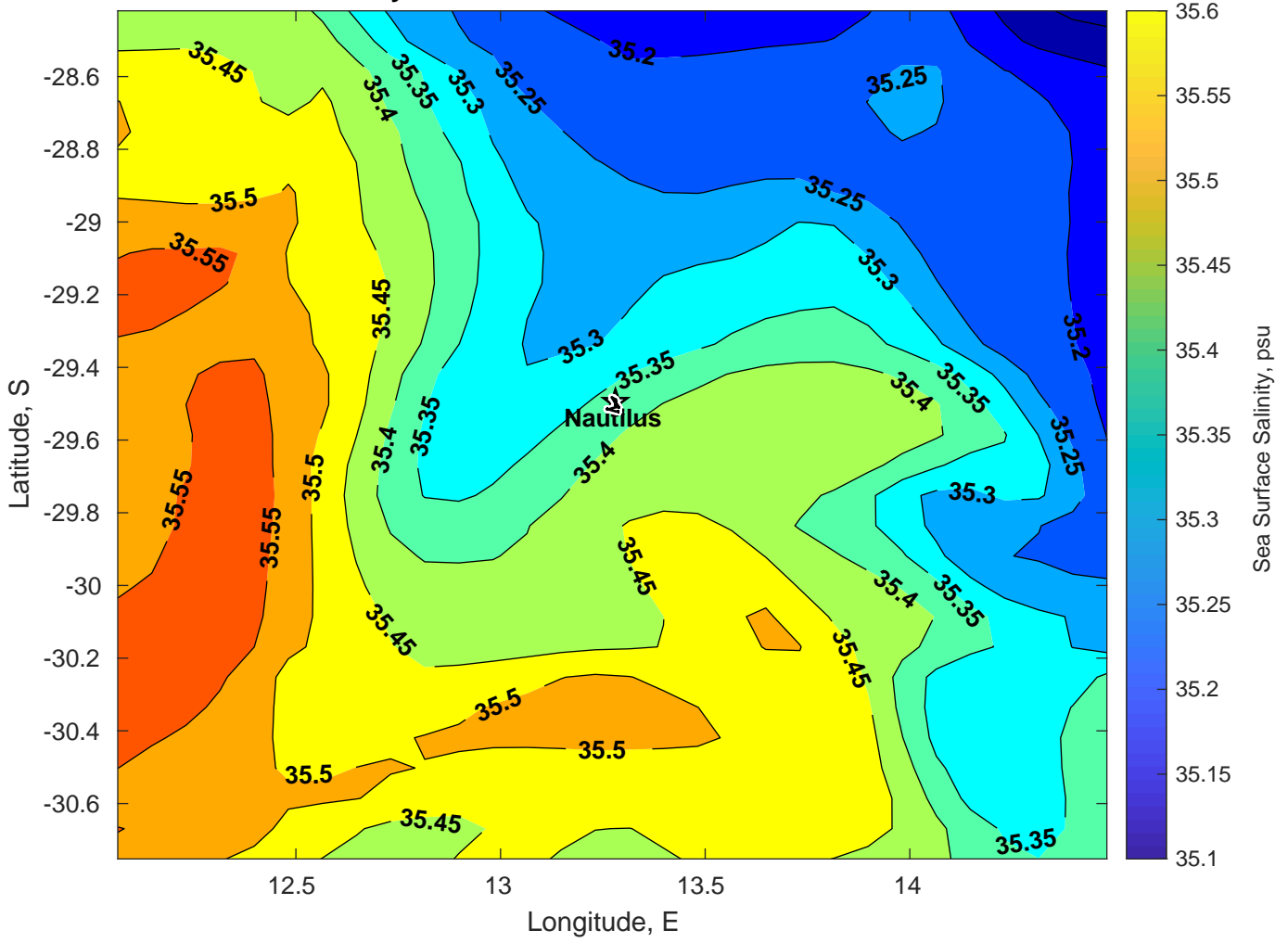
Surface Salinity for Nautilus at 09-Feb-2025 00:00:00
