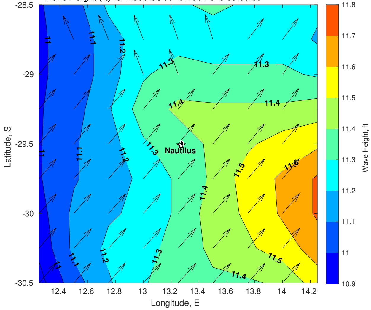
Wave Height (ft) for Nautilus at 10-Feb-2025 09:00:00
