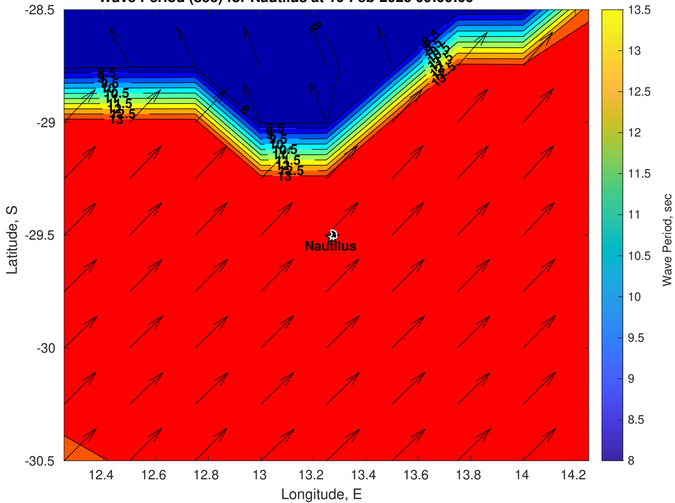
Wave Period (sec) for Nautilus at 10-Feb-2025 09:00:00
