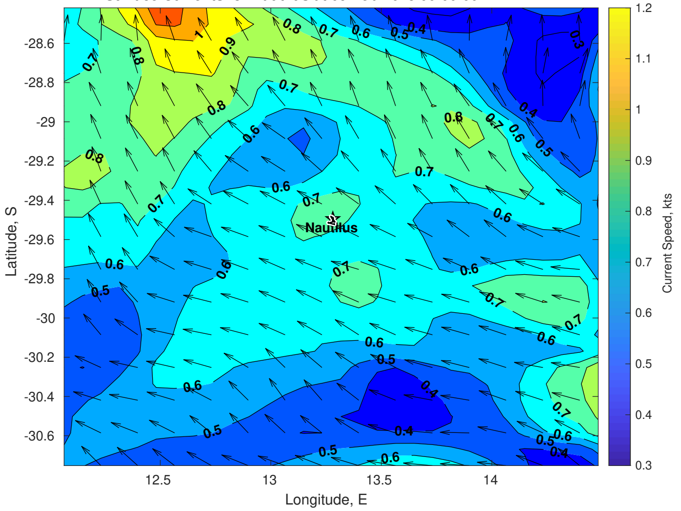
Surface Currents for Nautilus at 09-Feb-2025 00:00:00
