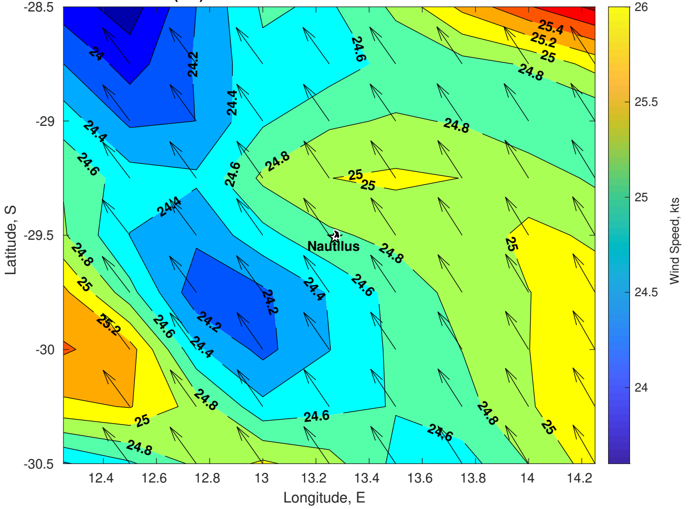
Winds (kts) for Nautilus at 10-Feb-2025 09:00:00
