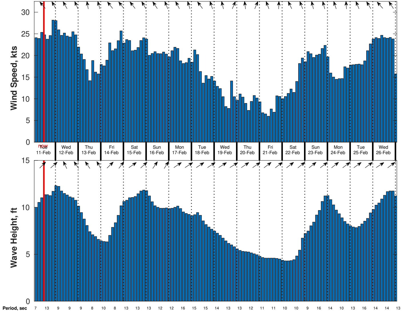
Wind & Wave Forecast for Nautilus from 10-Feb-2025 02:00:00 to 26-Feb-2025 02:00:00
