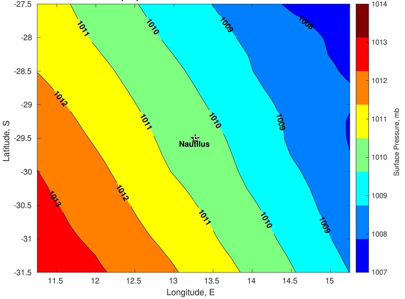
Surface Pressure (mb) for Nautilus at 12-Feb-2025 00:00:00
