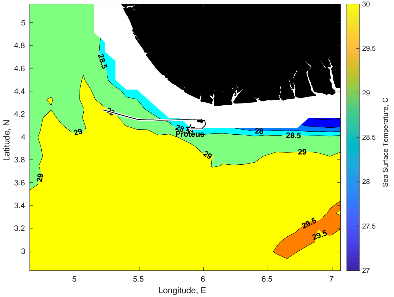
SST for Proteus at 09-Feb-2025 00:00:00
