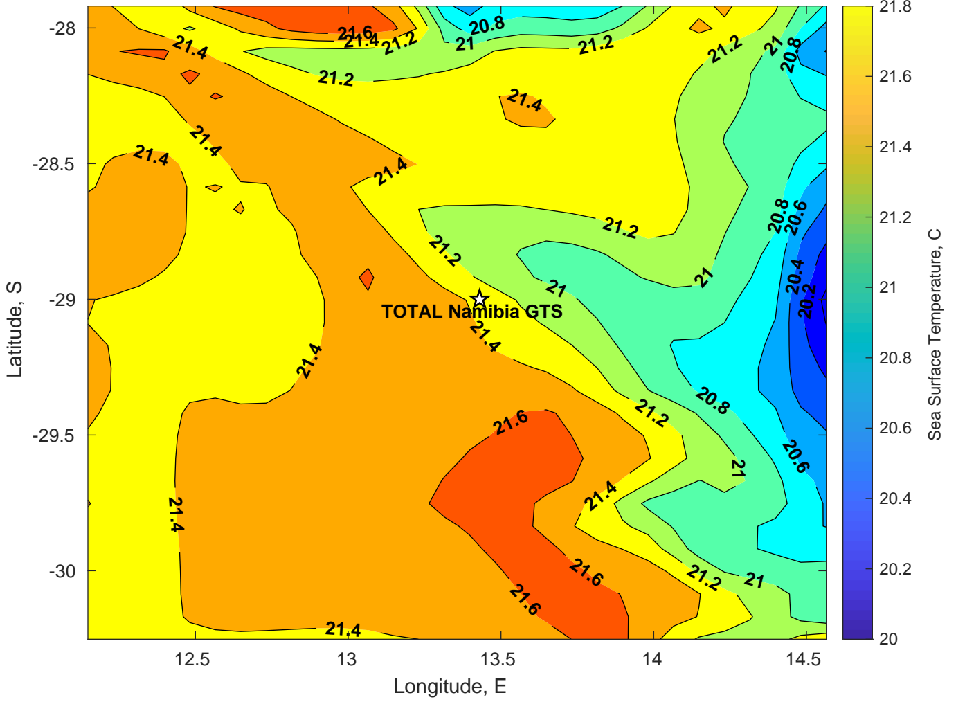
SST for TOTAL Namibia GTS at 09-Feb-2025 00:00:00
