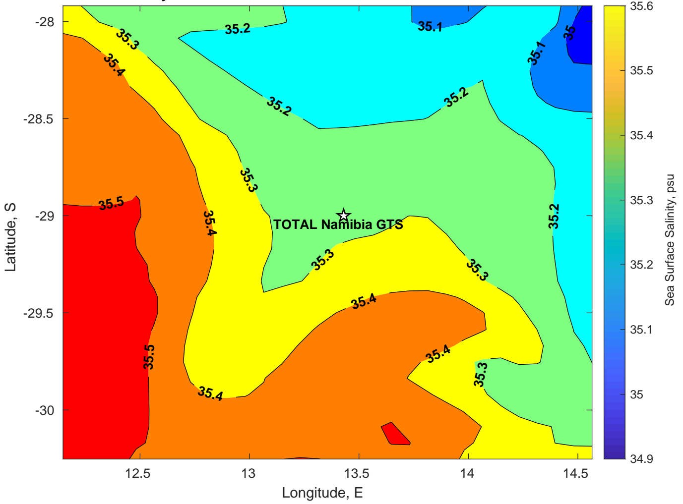
Surface Salinity for TOTAL Namibia GTS at 09-Feb-2025 00:00:00
