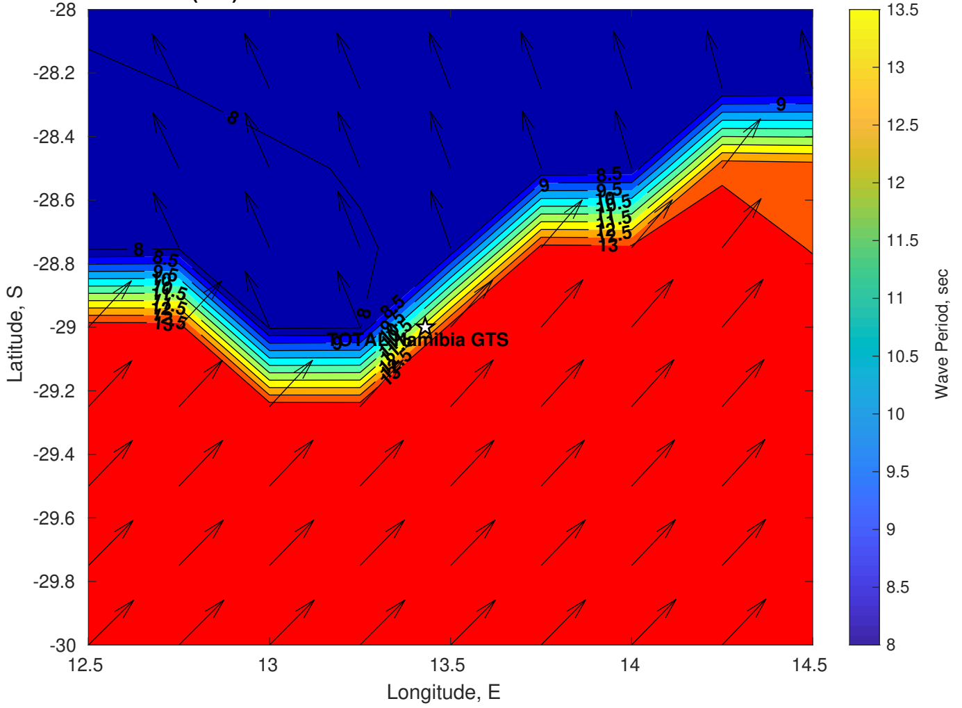
Wave Period (sec) for TOTAL Namibia GTS at 10-Feb-2025 09:00:00
