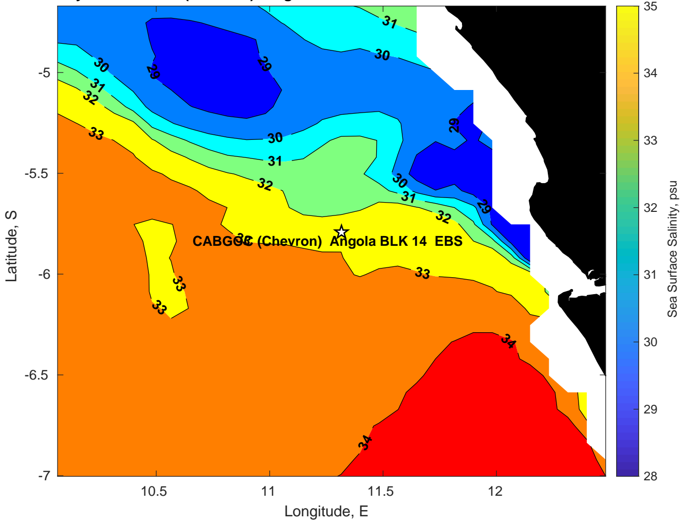
Surface Salinity for CABGOC (Chevron) Angola BLK 14 EBS at 10-Feb-2025 00:00:00
