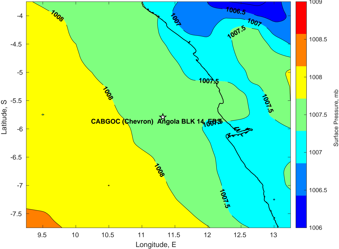
Surface Pressure (mb) for CABGOC (Chevron) Angola BLK 14 EBS at 10-Feb-2025 12:00:00
