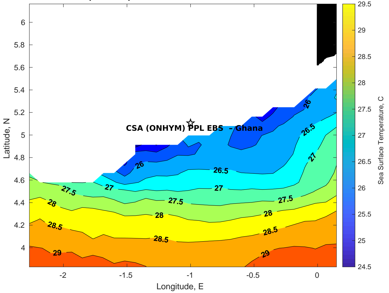
SST for CSA (ONHYM) PPL EBS - Ghana at 10-Feb-2025 00:00:00
