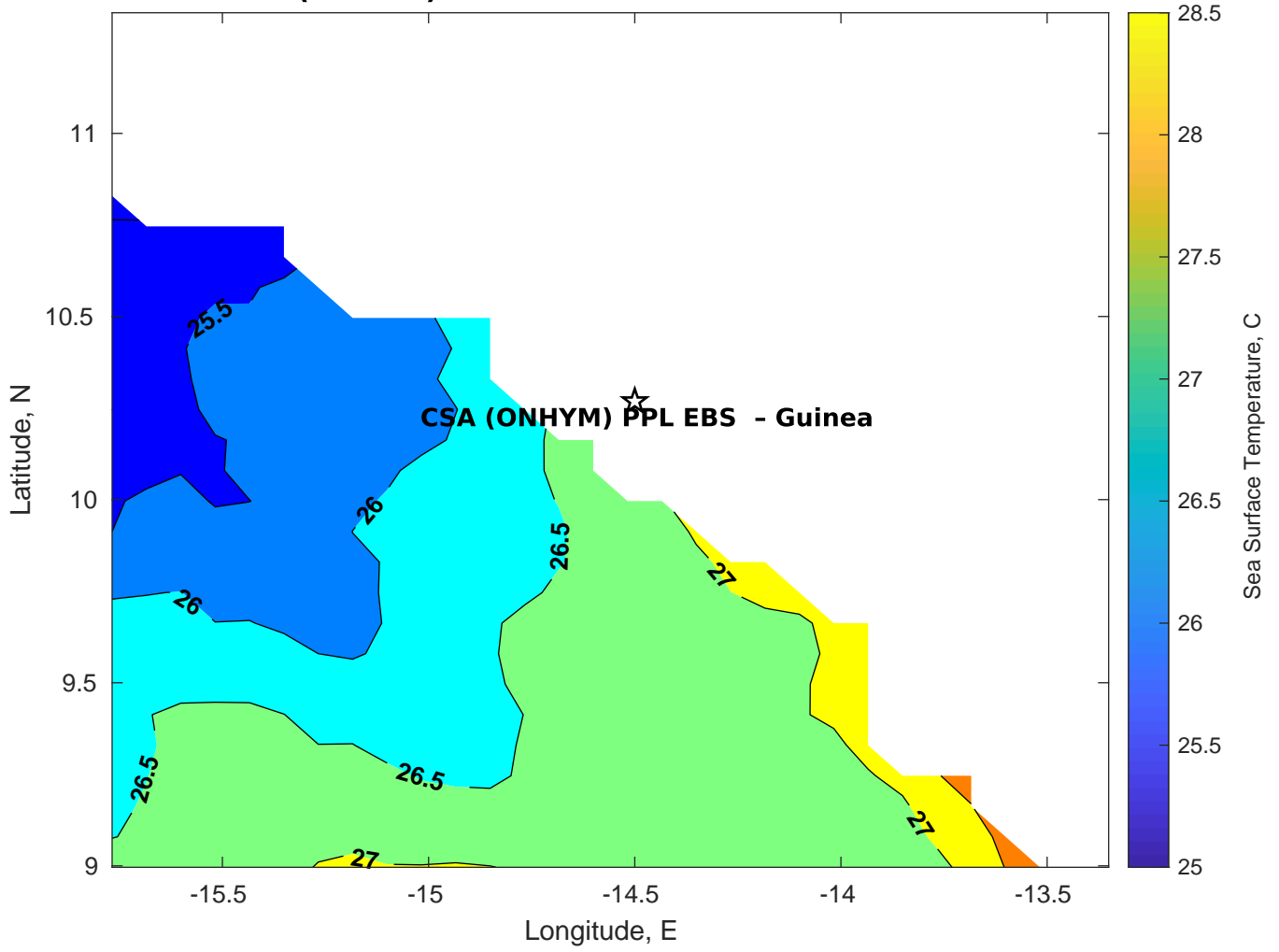
SST for CSA (ONHYM) PPL EBS - Guinea at 10-Feb-2025 00:00:00
