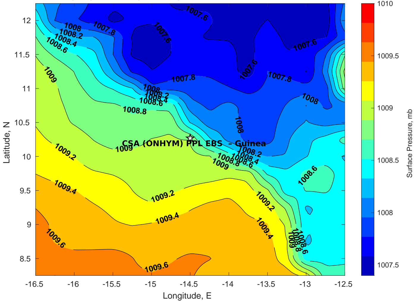
Surface Pressure (mb) for CSA (ONHYM) PPL EBS - Guinea at 11-Feb-2025 12:00:00
