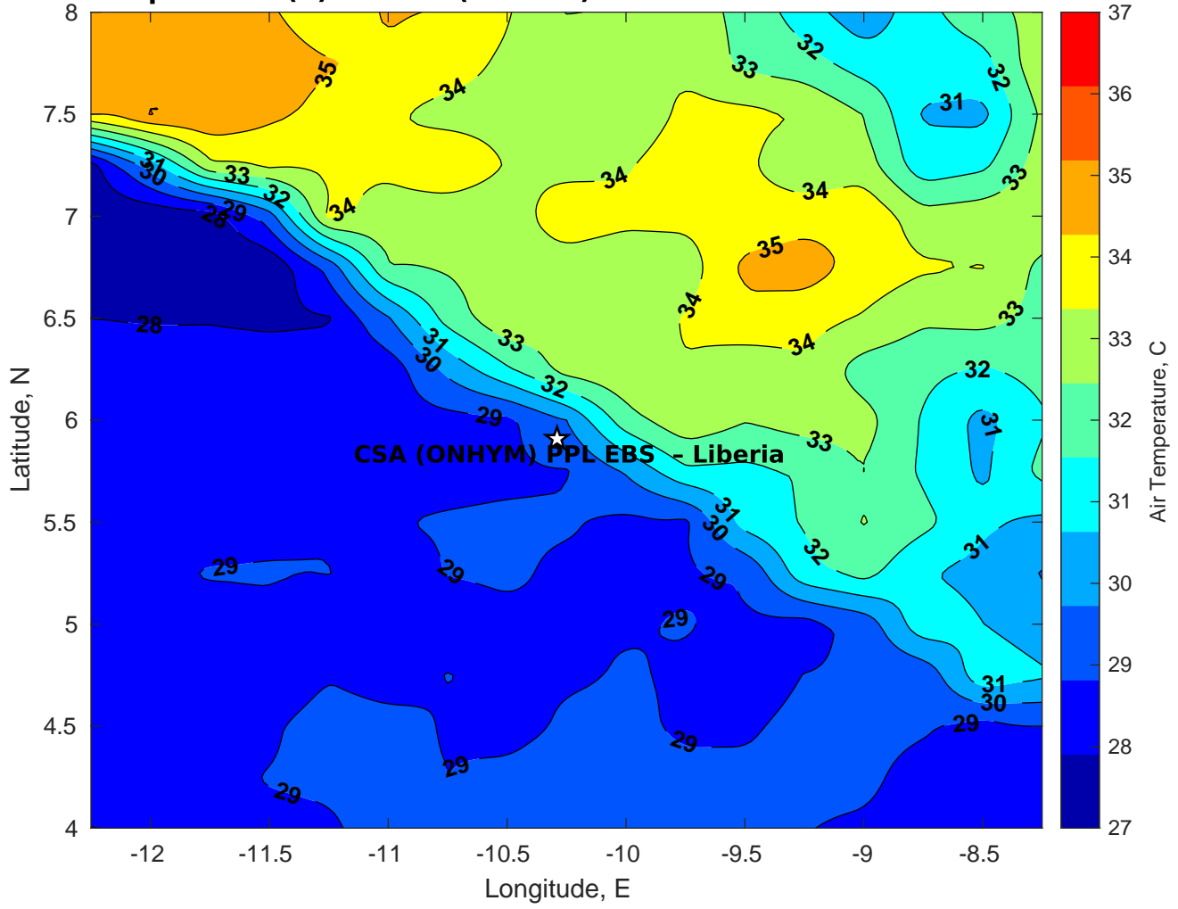
Air Temperature (C) for CSA (ONHYM) PPL EBS - Liberia at 10-Feb-2025
