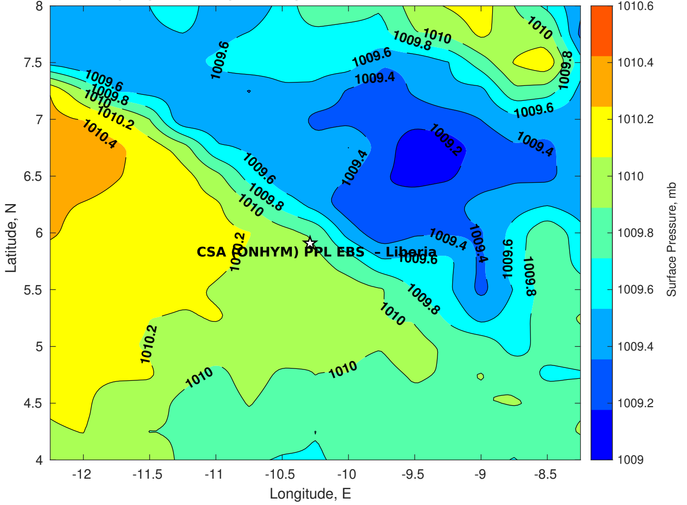
Surface Pressure (mb) for CSA (ONHYM) PPL EBS - Liberia at 12-Feb-2025 12:00:00
