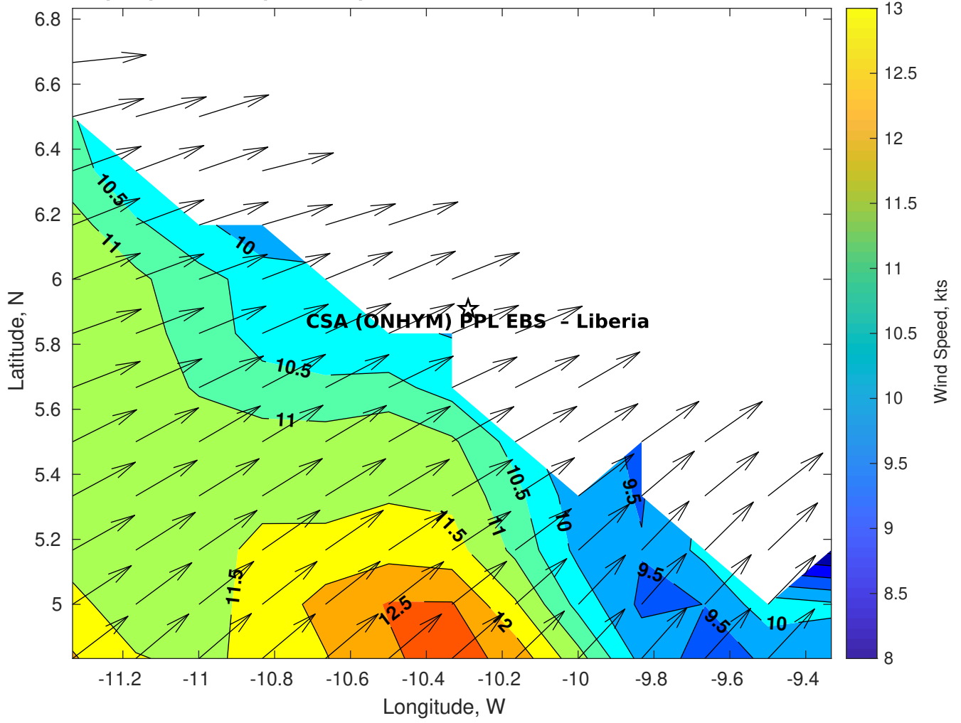
Winds (kts) for CSA (ONHYM) PPL EBS - Liberia at 10-Feb-2025 21:00:00
