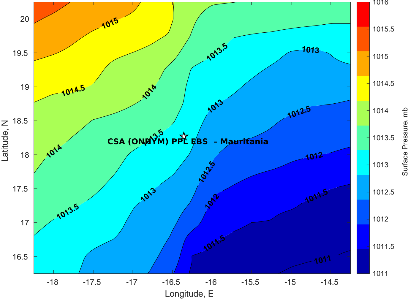
Surface Pressure (mb) for CSA (ONHYM) PPL EBS - Mauritania at 10-Feb-2025 12:00:00
