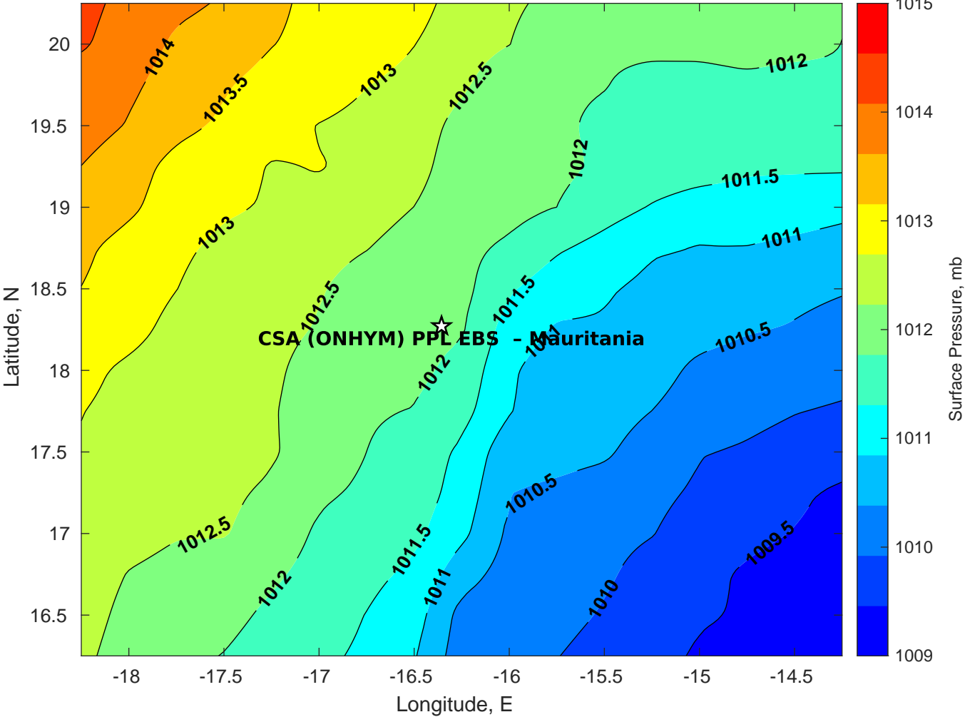
Surface Pressure (mb) for CSA (ONHYM) PPL EBS - Mauritania at 11-Feb-2025 12:00:00
