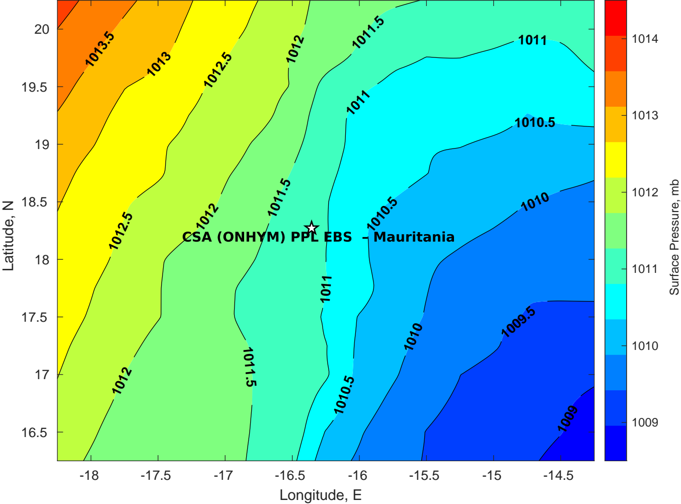
Surface Pressure (mb) for CSA (ONHYM) PPL EBS - Mauritania at 12-Feb-2025 12:00:00
