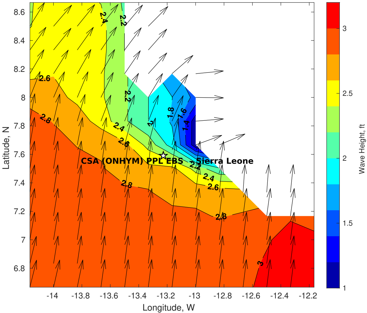
Wave Height (ft) for CSA (ONHYM) PPL EBS - Sierra Leone at 10-Feb-2025 21:00:00
