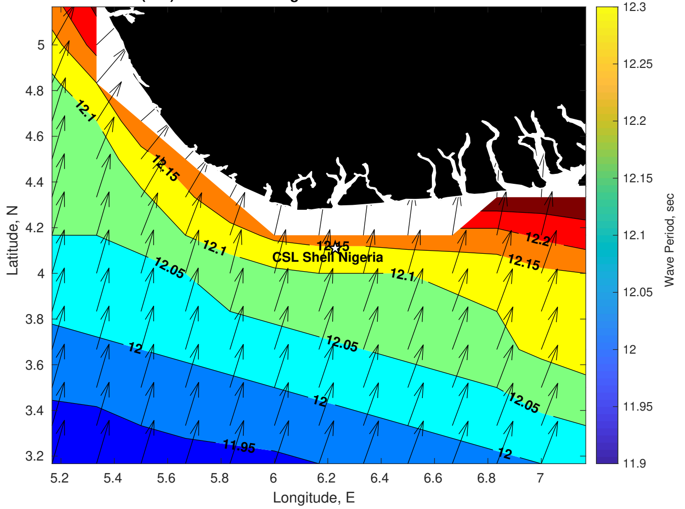
Wave Period (sec) for CSL Shell Nigeria at 10-Feb-2025 21:00:00
