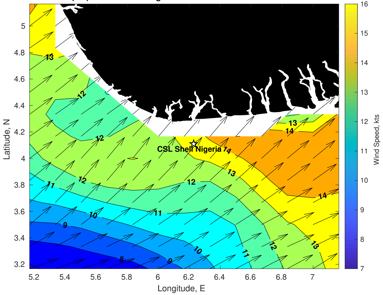
Winds (kts) for CSL Shell Nigeria at 10-Feb-2025 21:00:00
