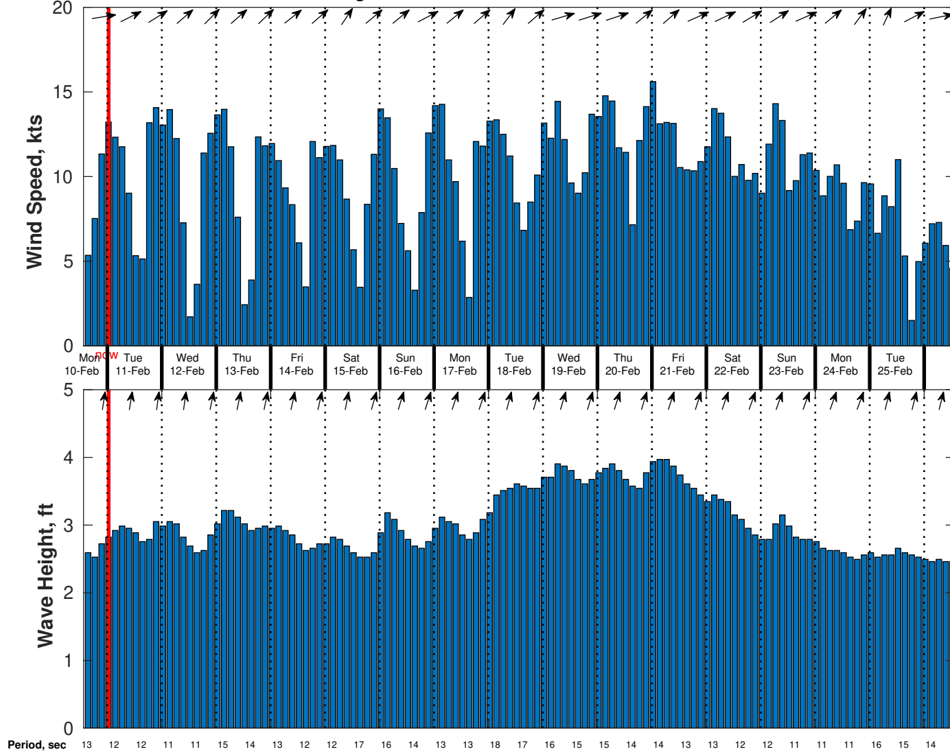
Wind & Wave Forecast for CSL Shell Nigeria from 10-Feb-2025 14:00:00 to 26-Feb-2025 14:00:00
