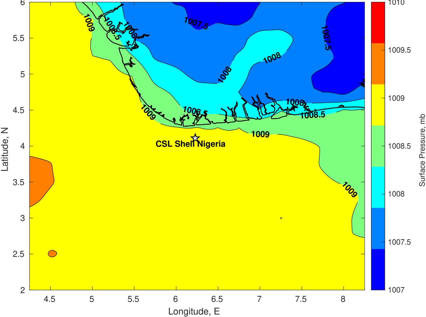
Surface Pressure (mb) for CSL Shell Nigeria at 12-Feb-2025 12:00:00
