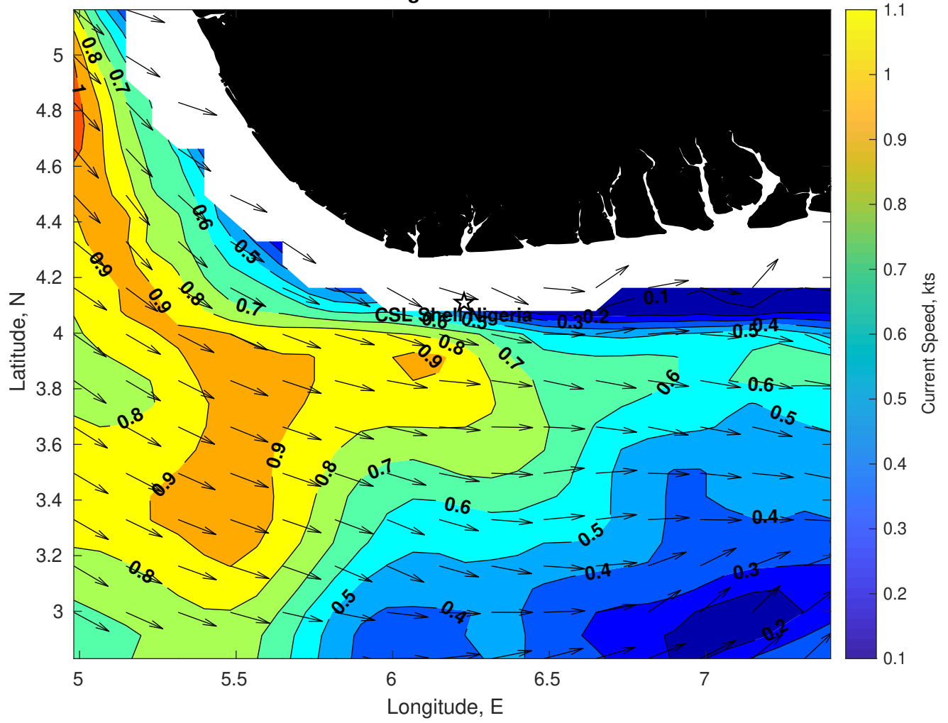
Surface Currents for CSL Shell Nigeria at 10-Feb-2025 00:00:00
