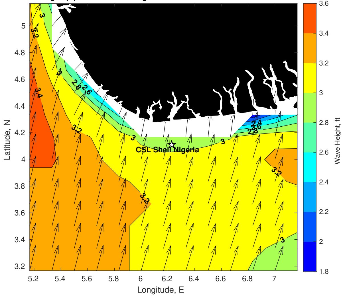
Wave Height (ft) for CSL Shell Nigeria at 10-Feb-2025 21:00:00
