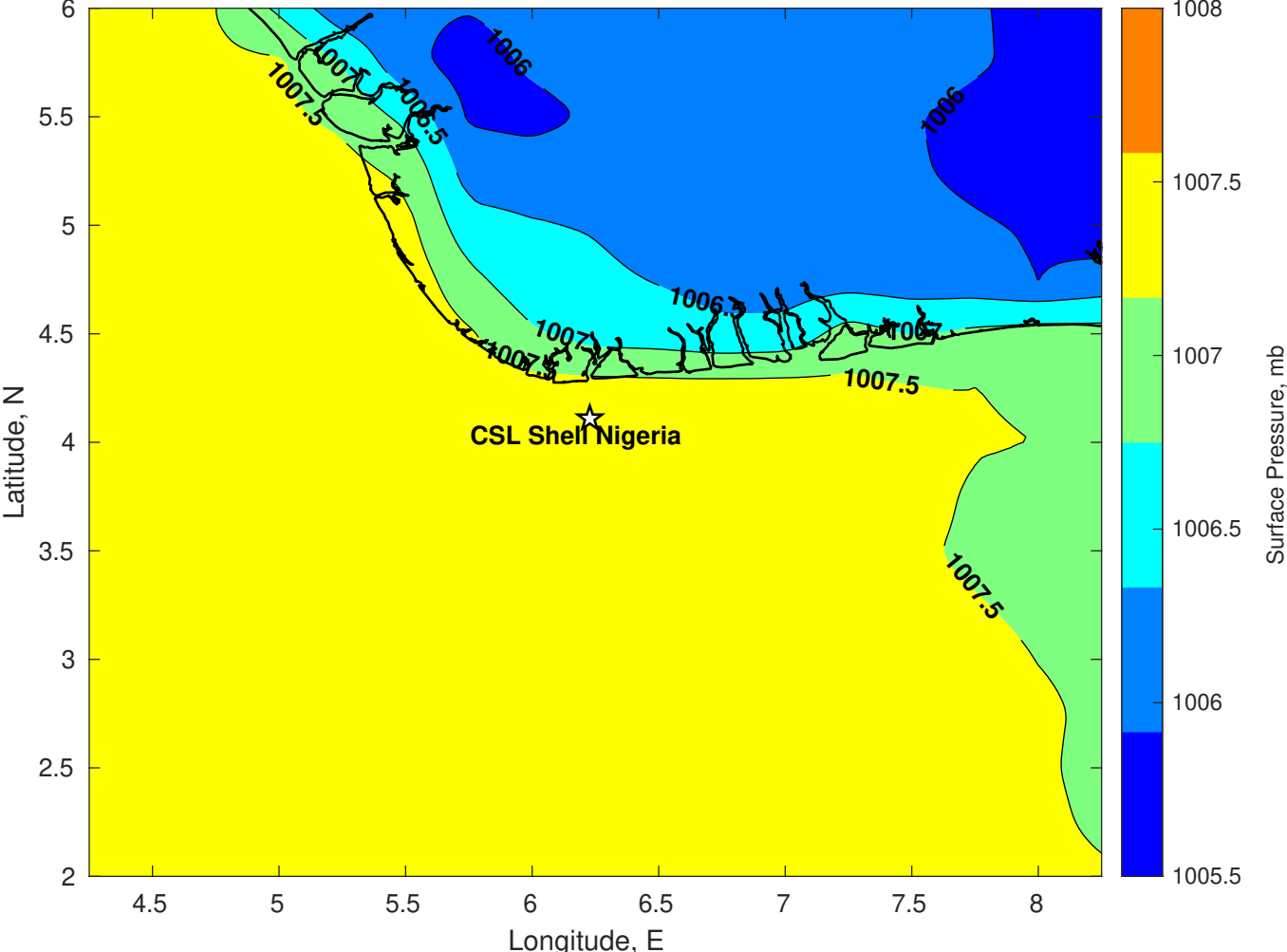
Surface Pressure (mb) for CSL Shell Nigeria at 11-Feb-2025 12:00:00
