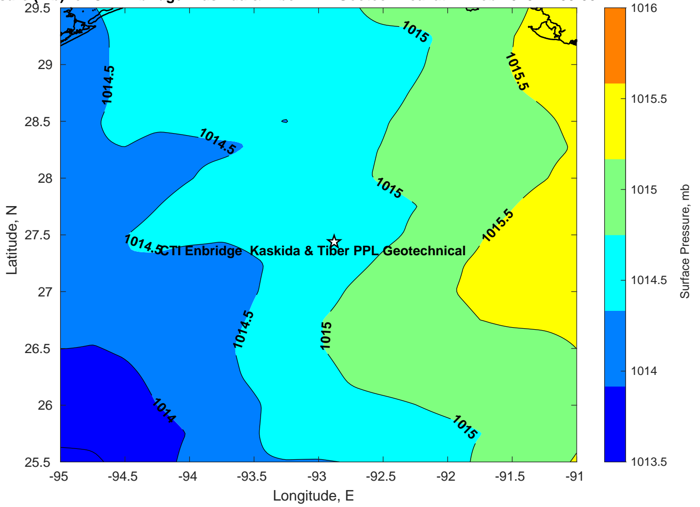
Surface Pressure (mb) for CTI Enbridge Kaskida & Tiber PPL Geotechnical at 11-Feb-2025 12:00:00
