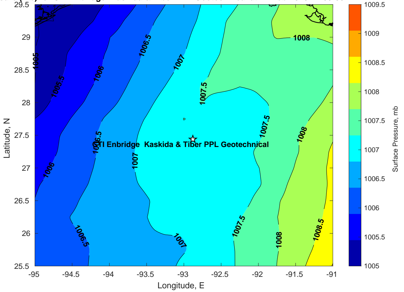
Surface Pressure (mb) for CTI Enbridge Kaskida & Tiber PPL Geotechnical at 12-Feb-2025 12:00:00
