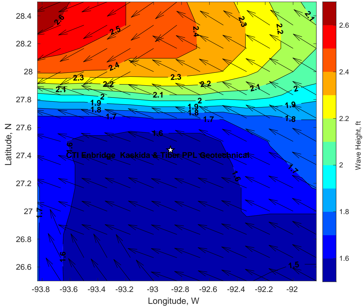
Wave Height (ft) for CTI Enbridge Kaskida & Tiber PPL Geotechnical at 10-Feb-2025 21:00:00
