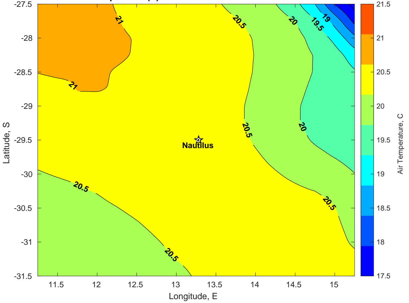
Air Temperature (C) for Nautilus at 10-Feb-2025
