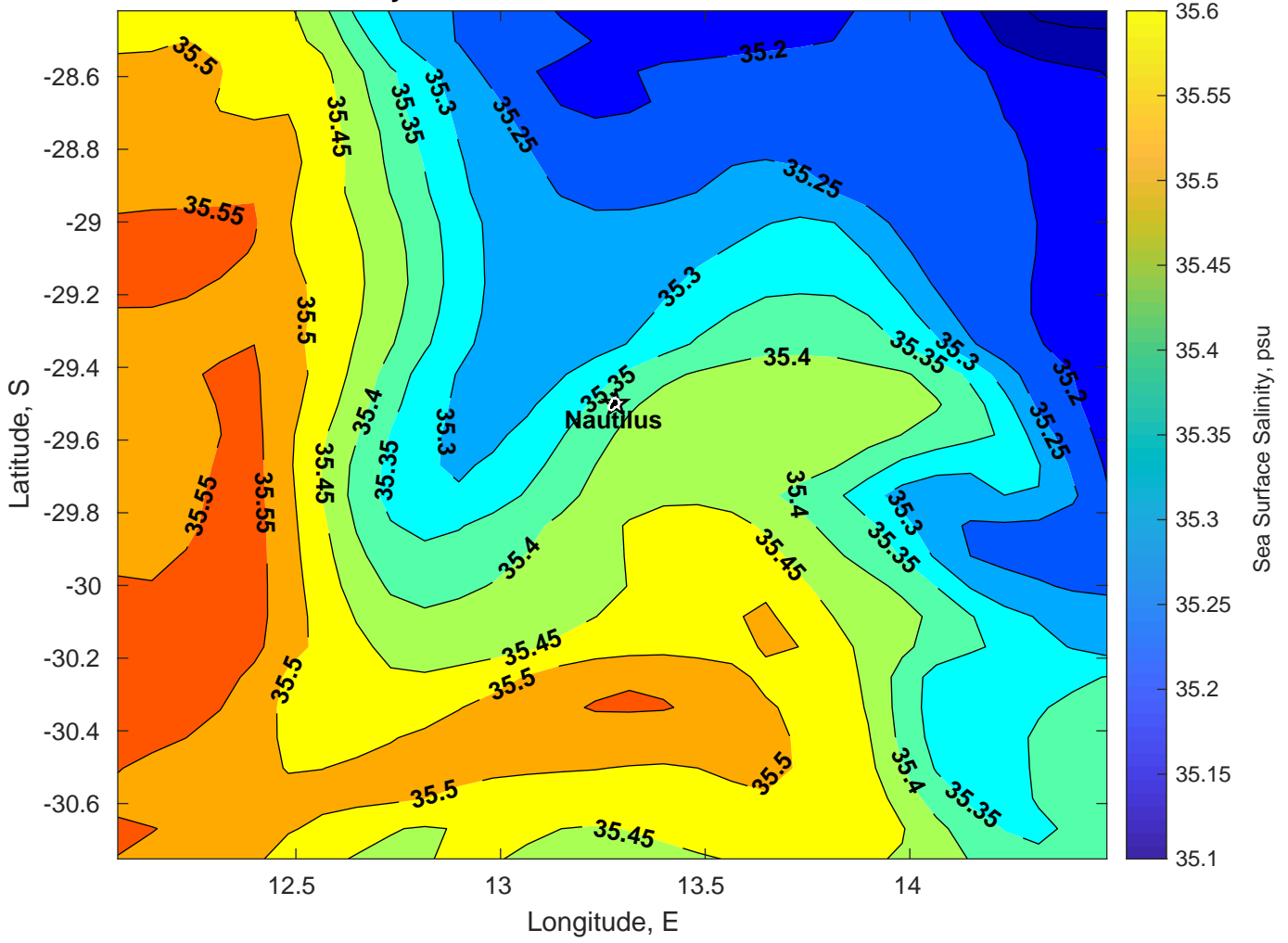
Surface Salinity for Nautilus at 10-Feb-2025 00:00:00
