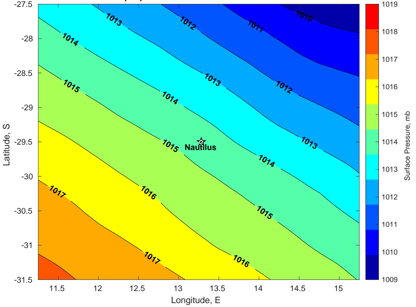
Surface Pressure (mb) for Nautilus at 10-Feb-2025 12:00:00
