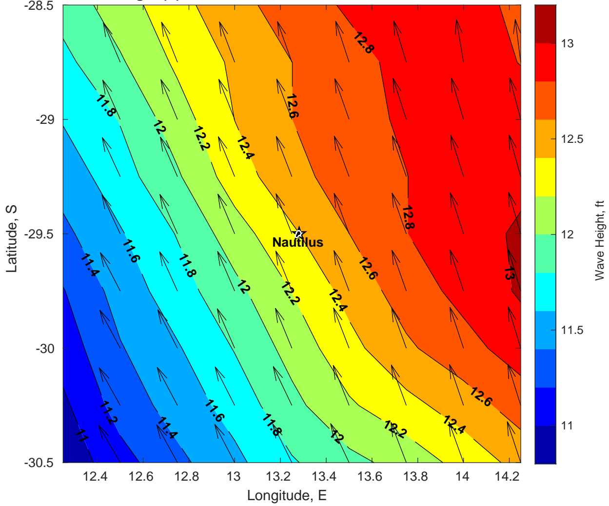
Wave Height (ft) for Nautilus at 10-Feb-2025 21:00:00
