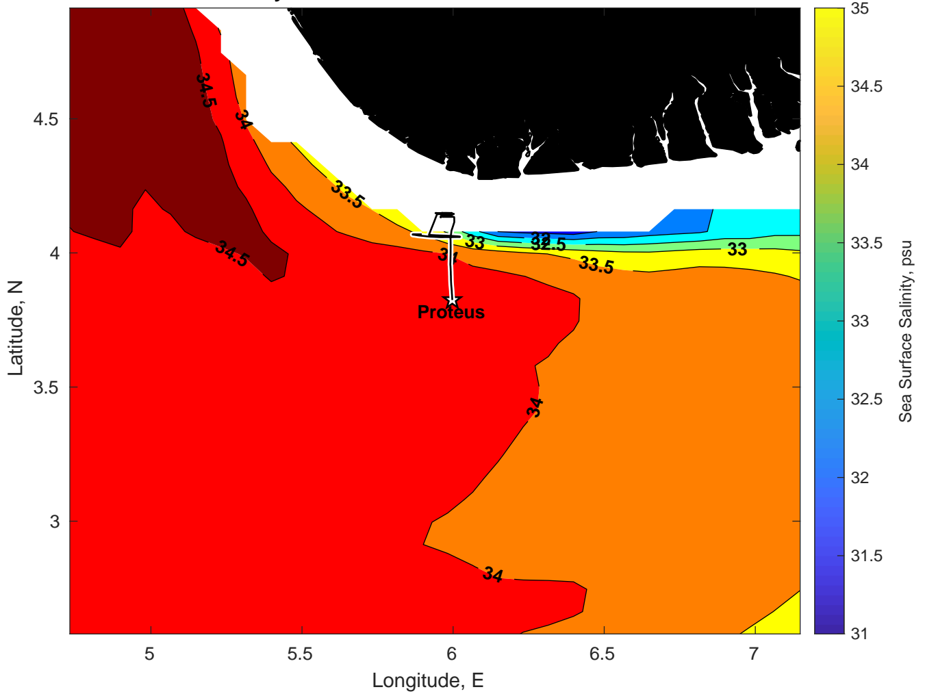
Surface Salinity for Proteus at 10-Feb-2025 00:00:00
