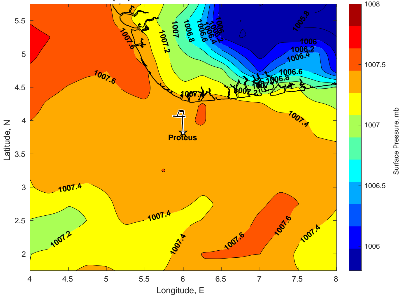
Surface Pressure (mb) for Proteus at 10-Feb-2025 12:00:00
