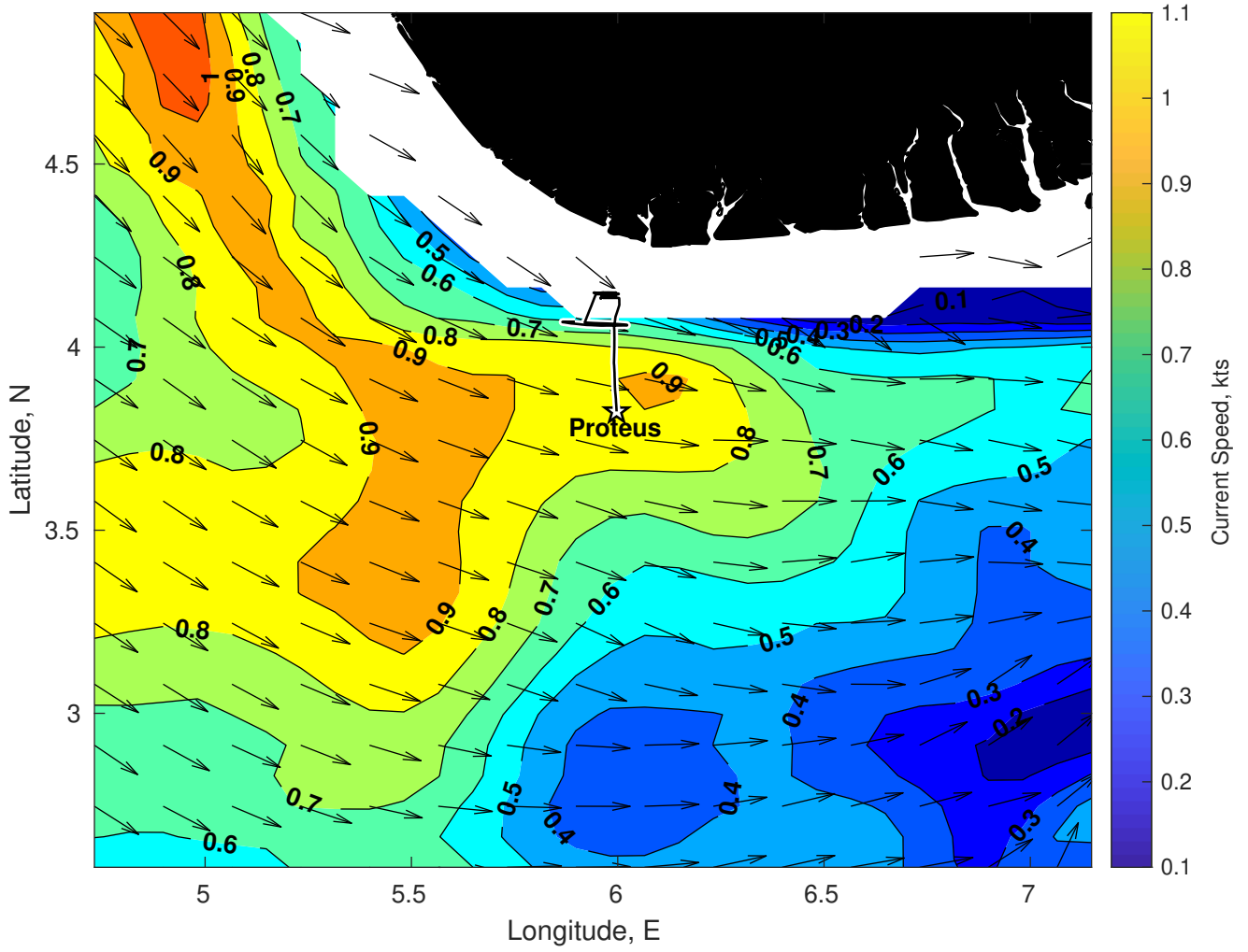
Surface Currents for Proteus at 10-Feb-2025 00:00:00
