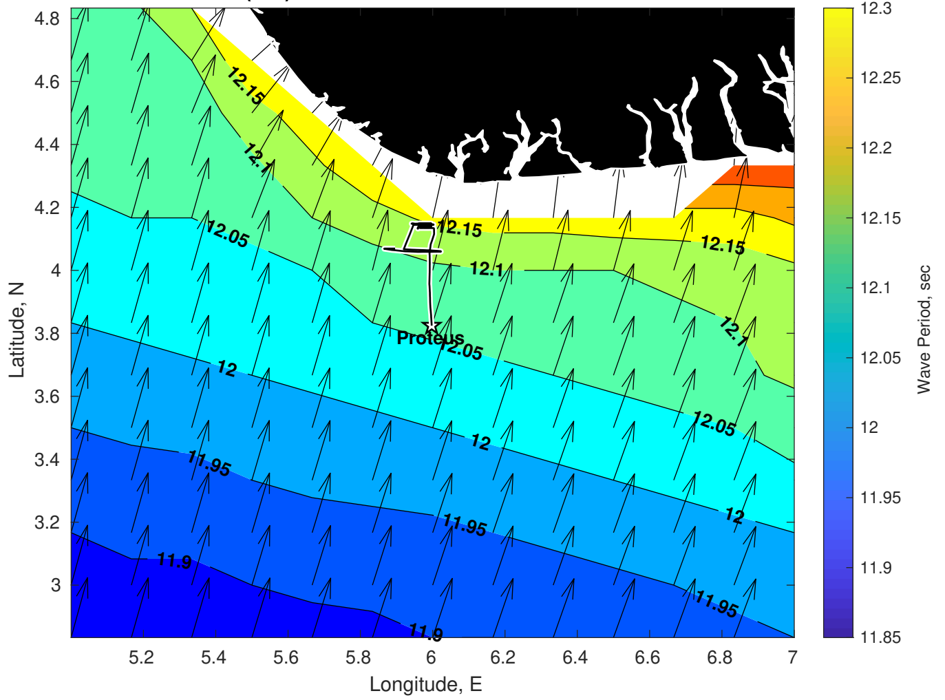
Wave Period (sec) for Proteus at 10-Feb-2025 21:00:00
