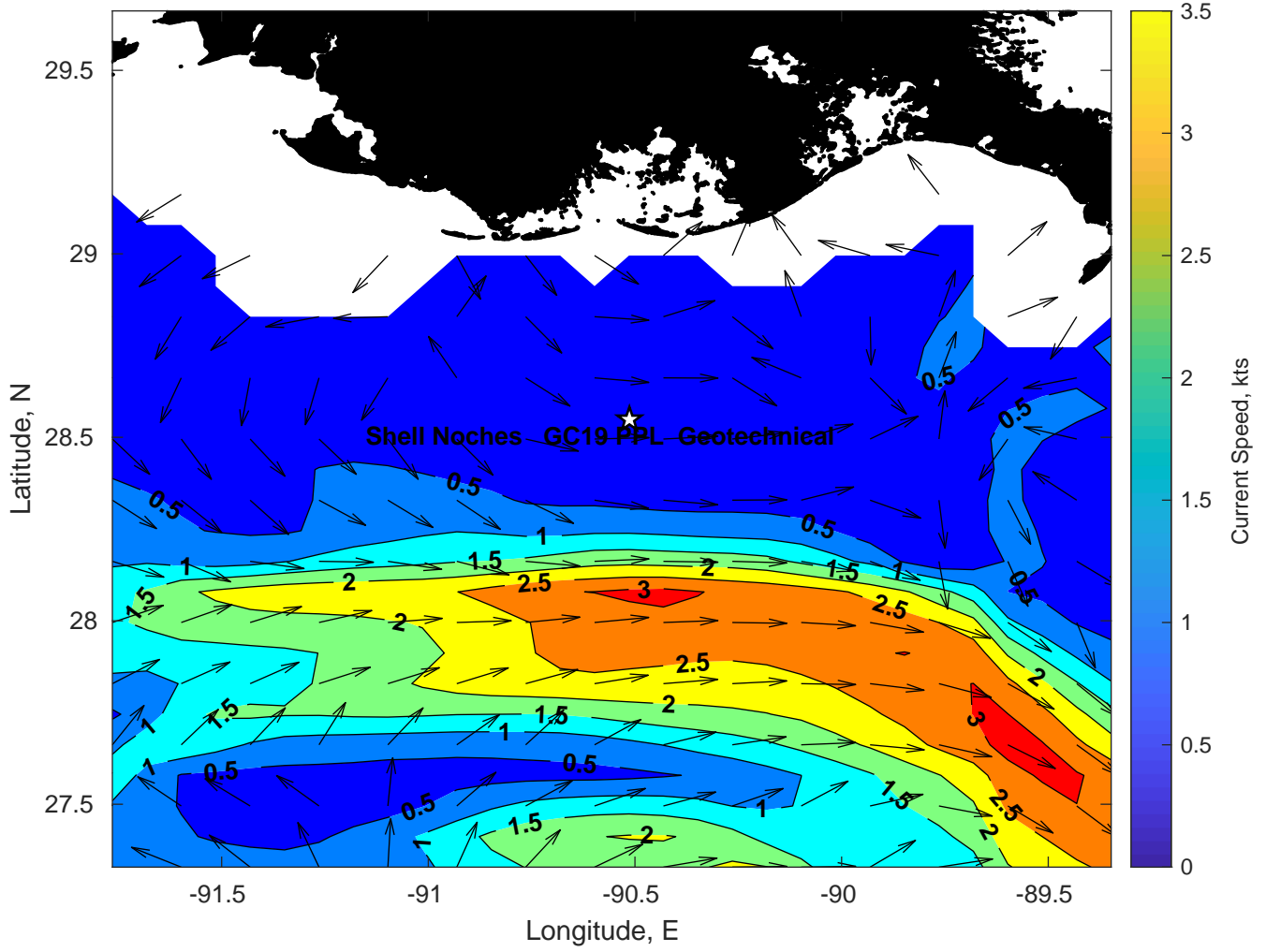
Surface Currents for Shell Noches GC19 PPL Geotechnical at 10-Feb-2025 00:00:00
