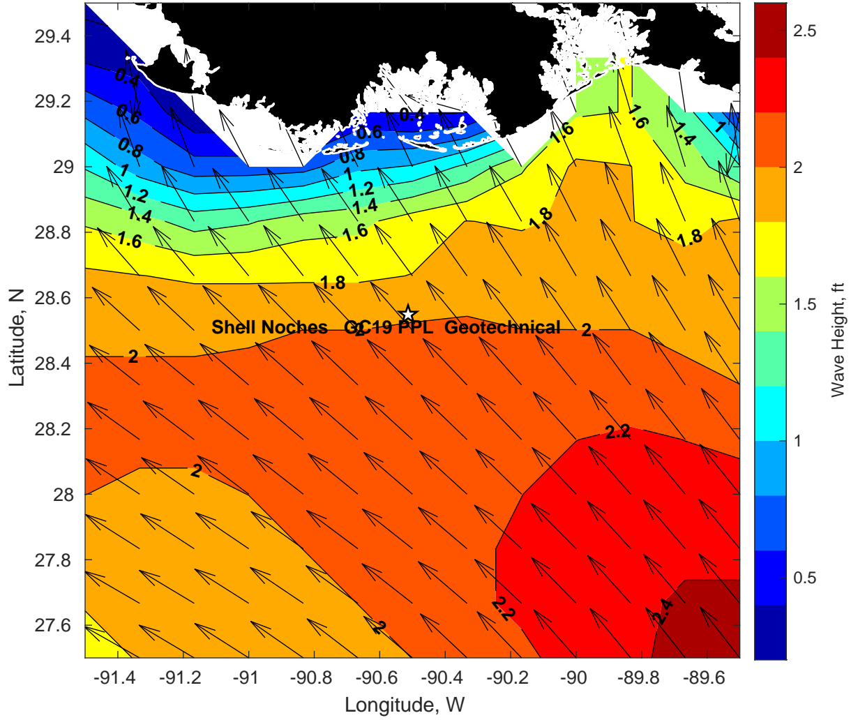
Wave Height (ft) for Shell Noches GC19 PPL Geotechnical at 10-Feb-2025 21:00:00
