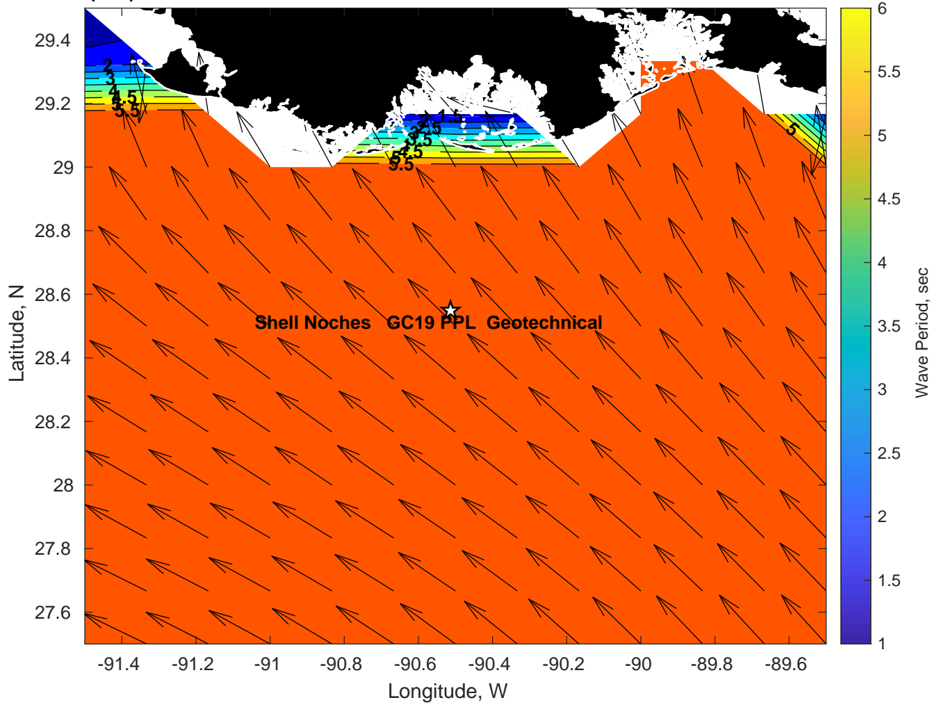
Wave Period (sec) for Shell Noches GC19 PPL Geotechnical at 10-Feb-2025 21:00:00
