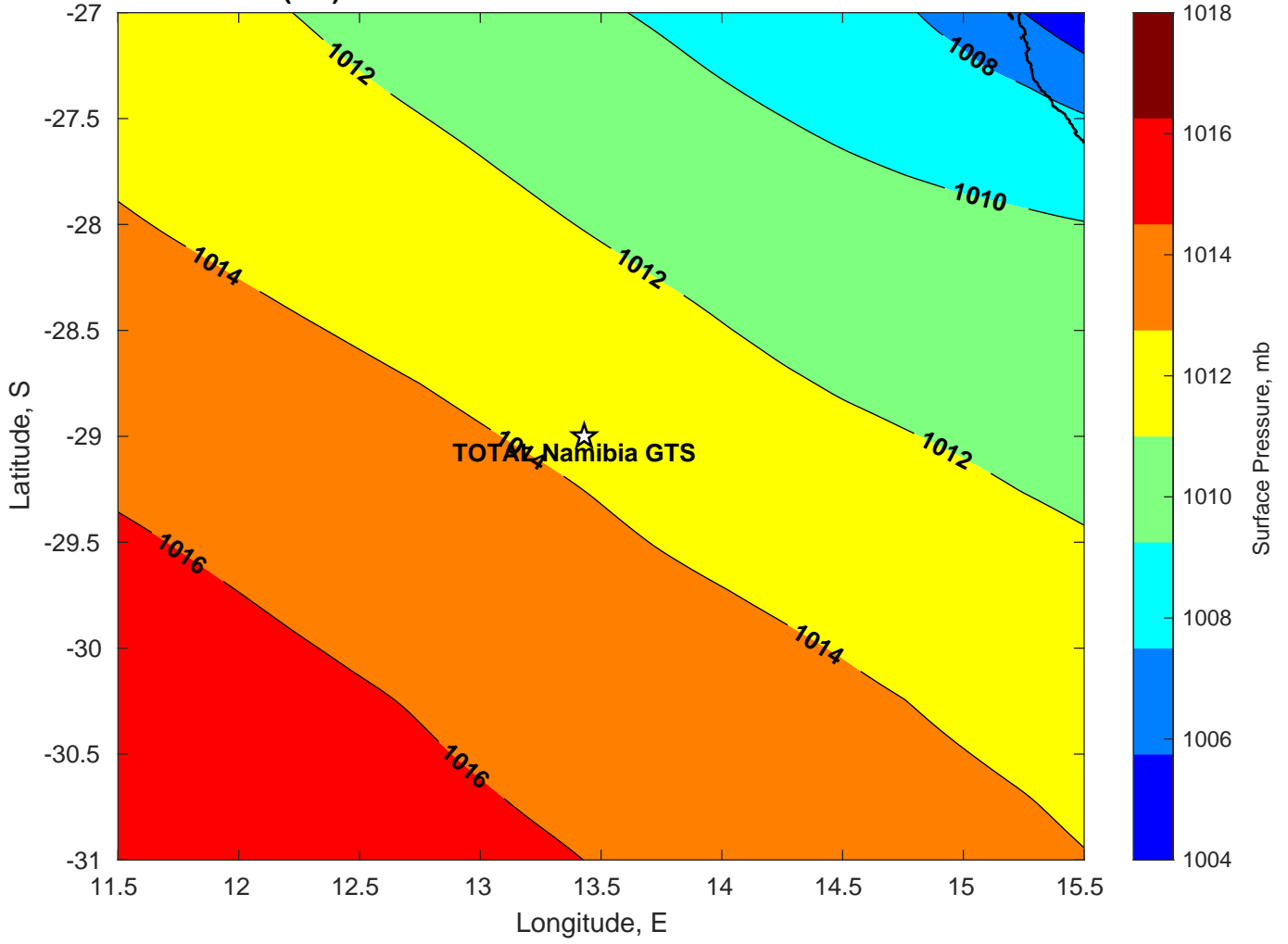
Surface Pressure (mb) for TOTAL Namibia GTS at 10-Feb-2025 12:00:00
