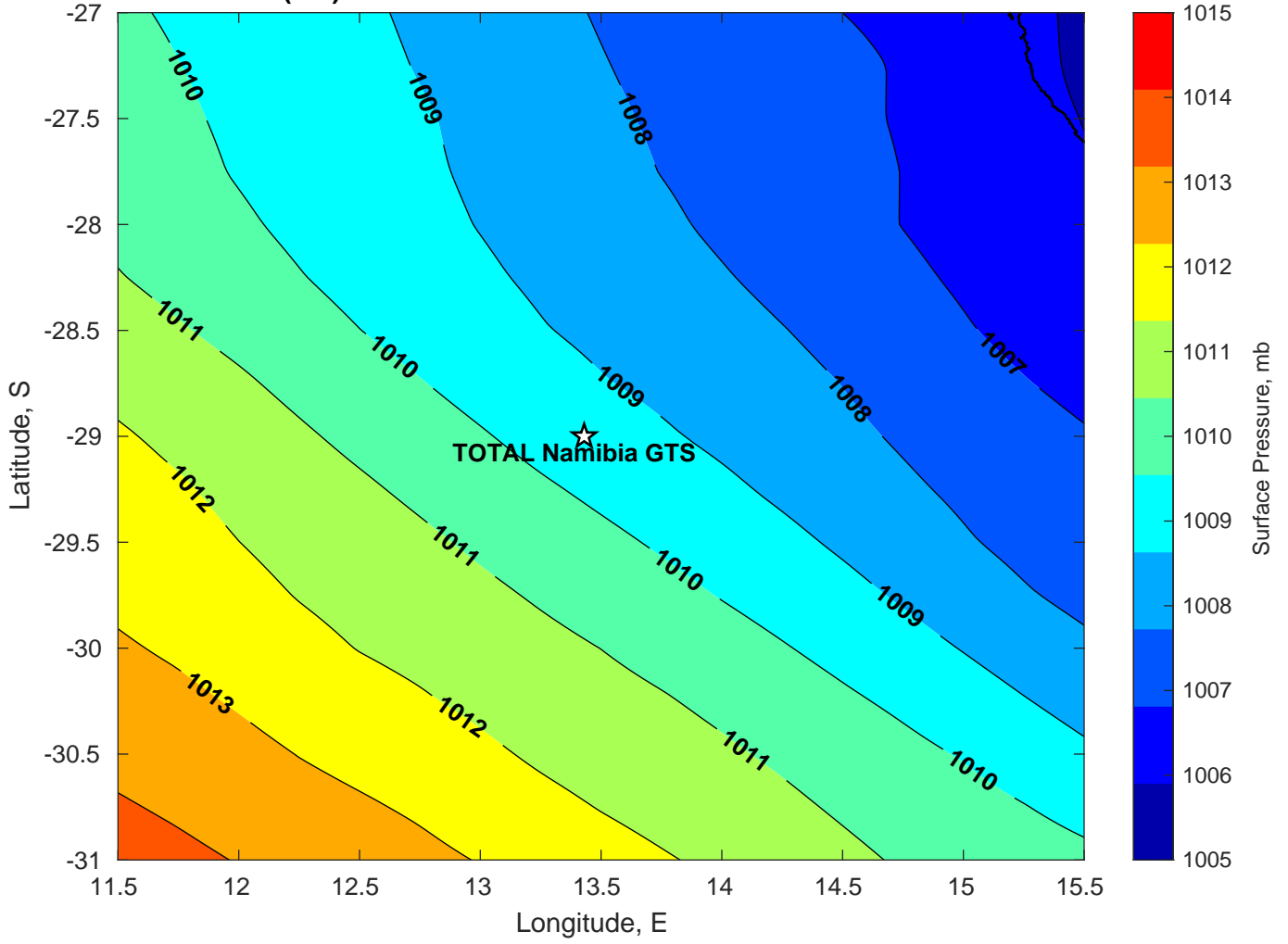
Surface Pressure (mb) for TOTAL Namibia GTS at 11-Feb-2025 12:00:00
