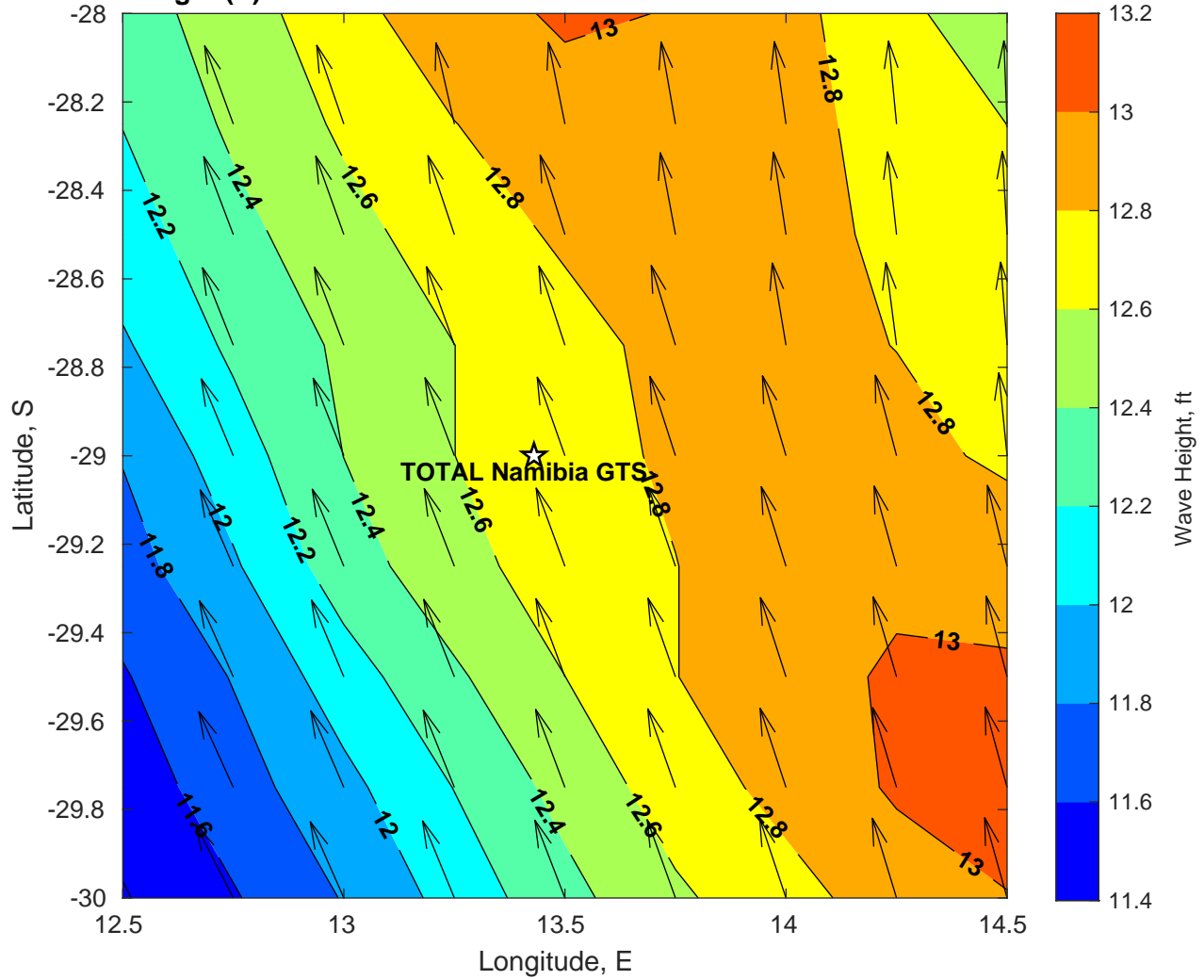
Wave Height (ft) for TOTAL Namibia GTS at 10-Feb-2025 21:00:00
