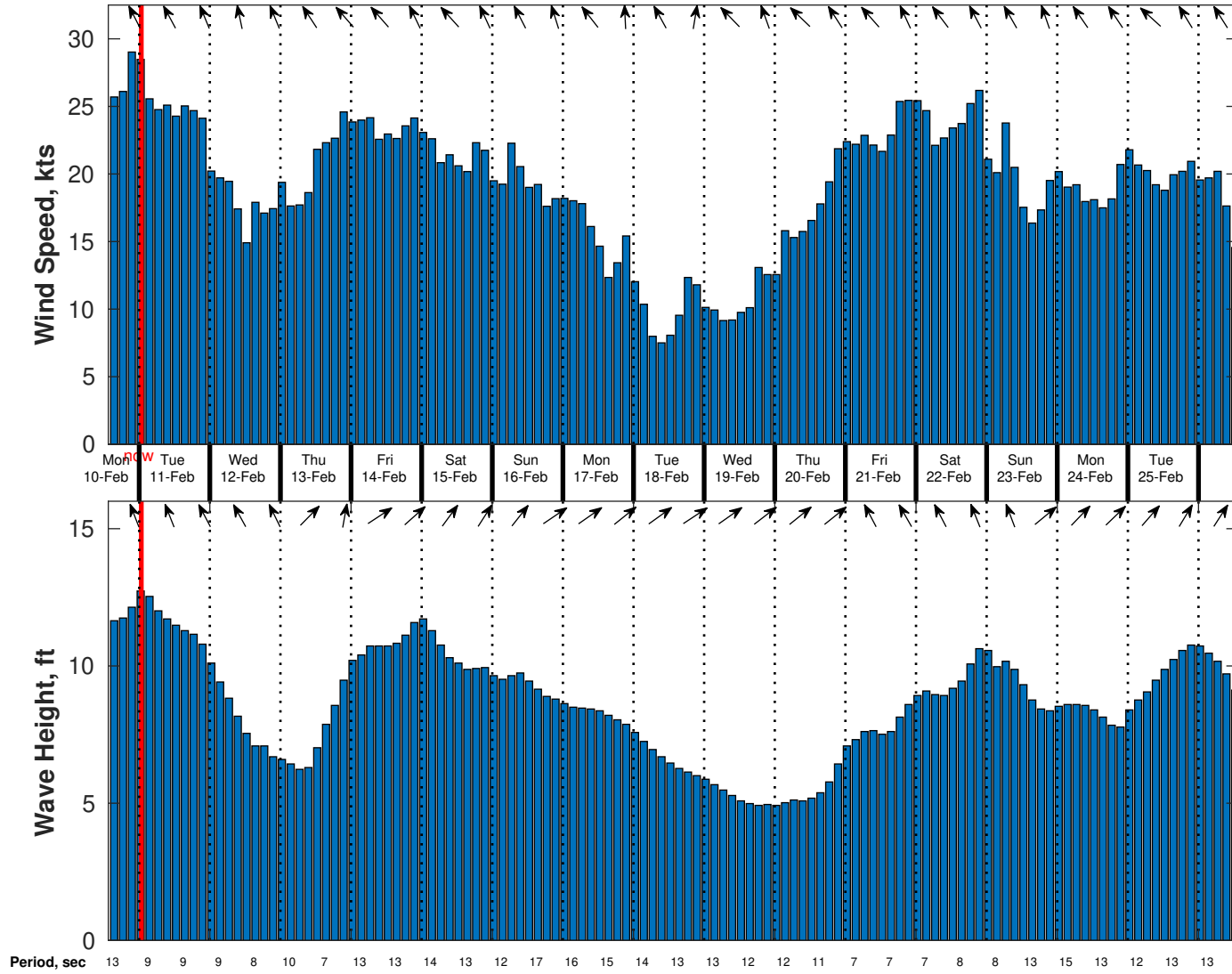
Wind & Wave Forecast for TOTAL Namibia GTS from 10-Feb-2025 14:00:00 to 26-Feb-2025 14:00:00
