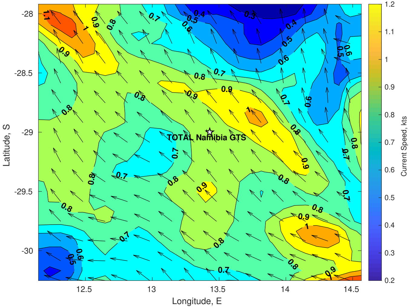
Surface Currents for TOTAL Namibia GTS at 10-Feb-2025 00:00:00
