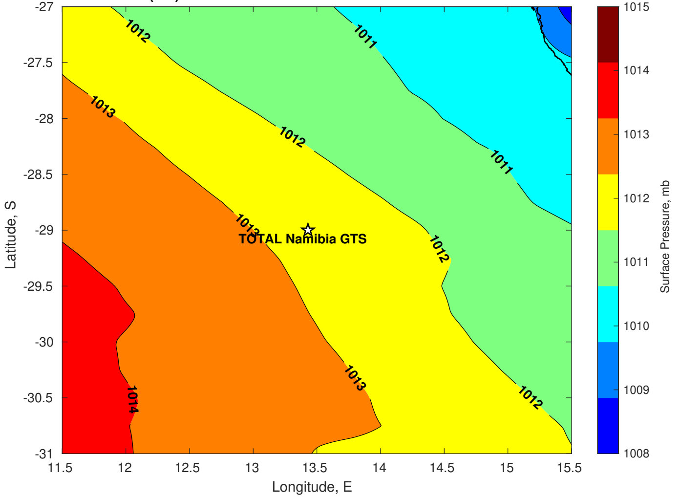
Surface Pressure (mb) for TOTAL Namibia GTS at 12-Feb-2025 12:00:00
