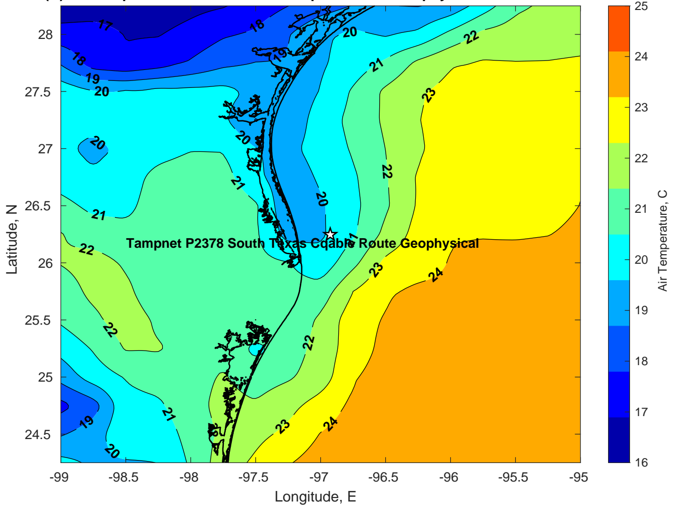
Air Temperature (C) for Tampnet P2378 South Texas Cqable Route Geophysical at 10-Feb-2025
