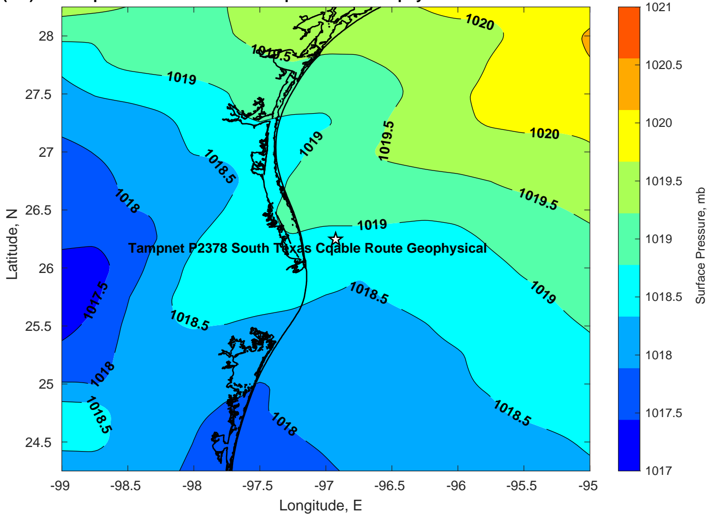
Pressure (mb) for Tampnet P2378 South Texas Cqable Route Geophysical at 10-Feb-2025 12:00:00
