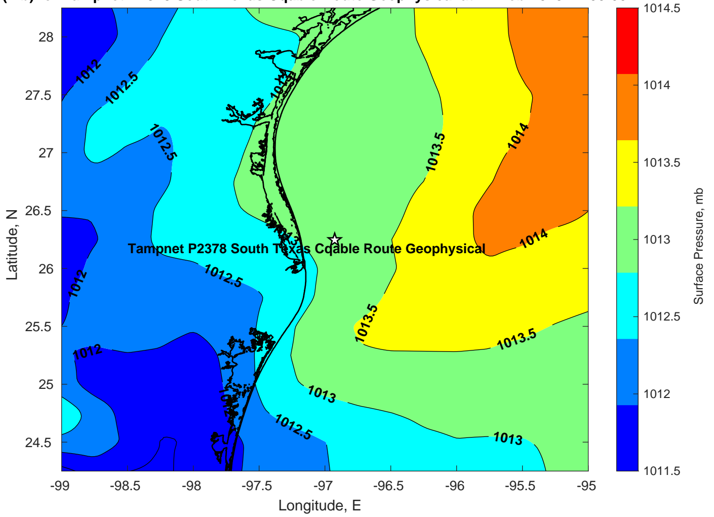
Pressure (mb) for Tampnet P2378 South Texas Cqable Route Geophysical at 11-Feb-2025 12:00:00
