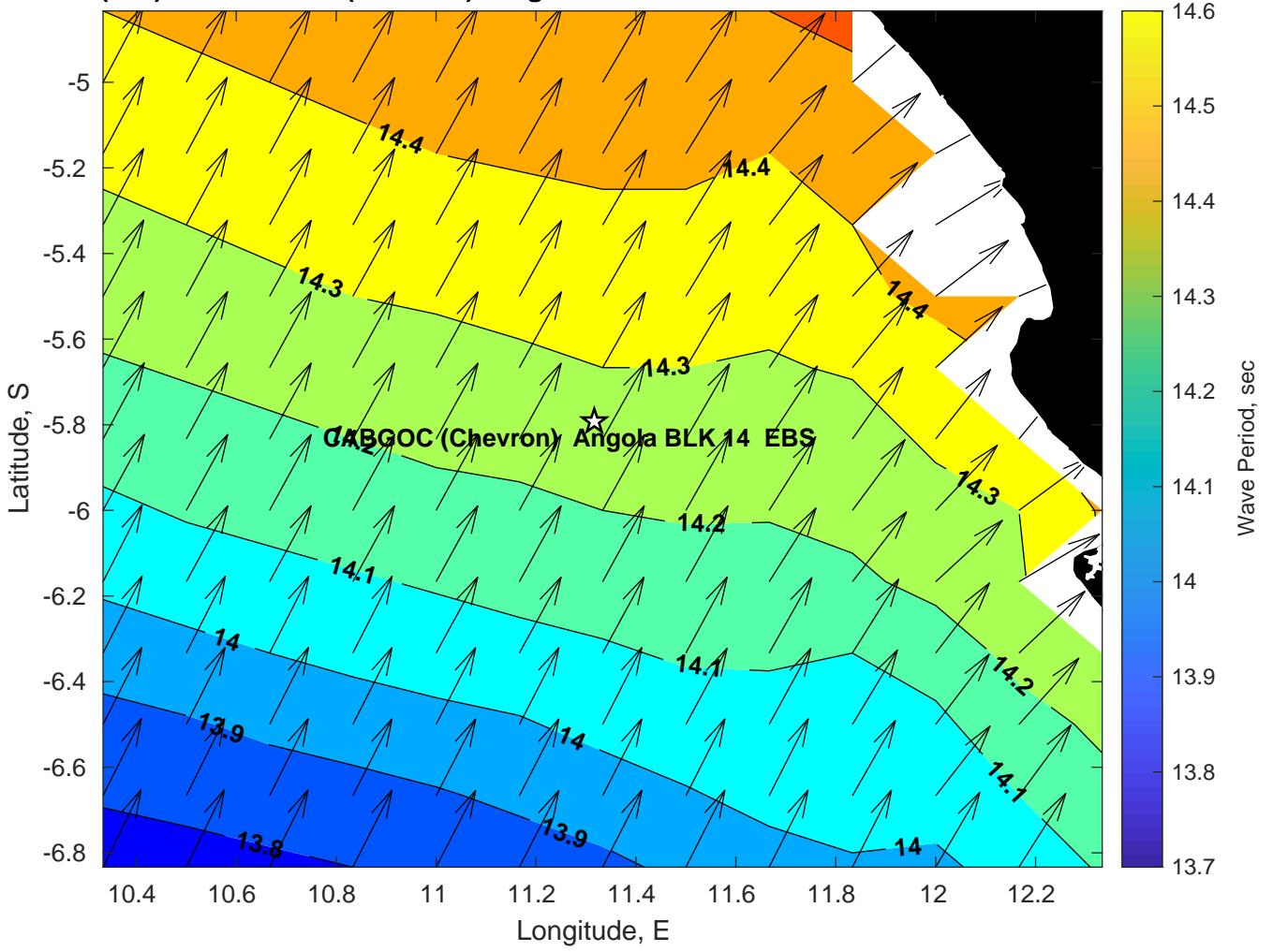
Wave Period (sec) for CABGOC (Chevron) Angola BLK 14 EBS at 12-Feb-2025 09:00:00
