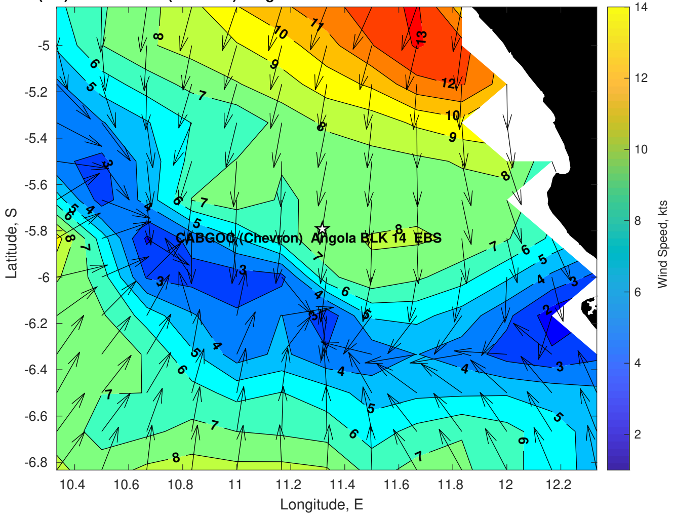
Winds (kts) for CABGOC (Chevron) Angola BLK 14 EBS at 12-Feb-2025 09:00:00
