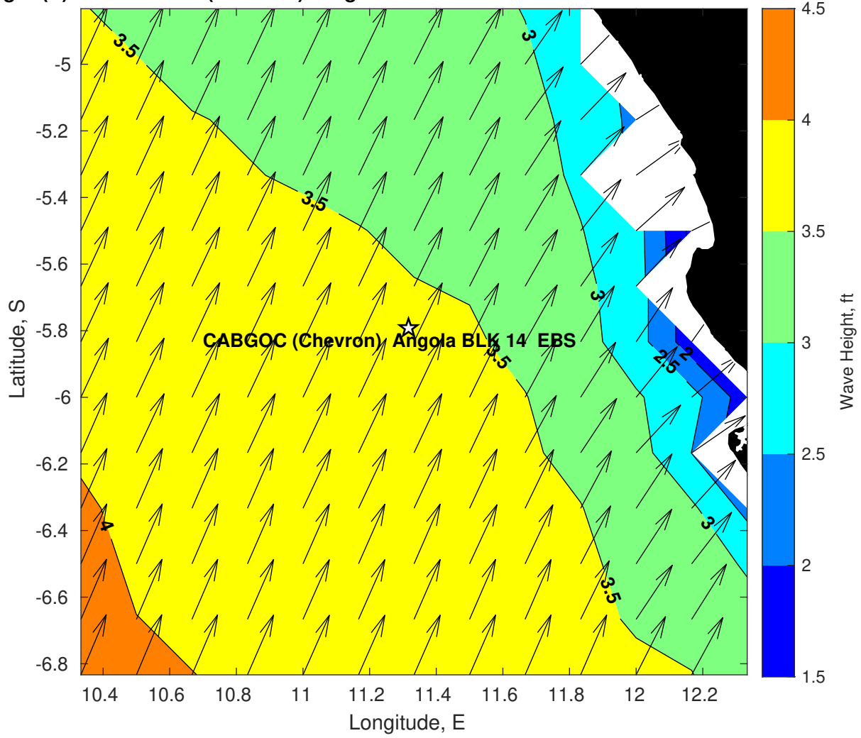
Wave Height (ft) for CABGOC (Chevron) Angola BLK 14 EBS at 12-Feb-2025 09:00:00
