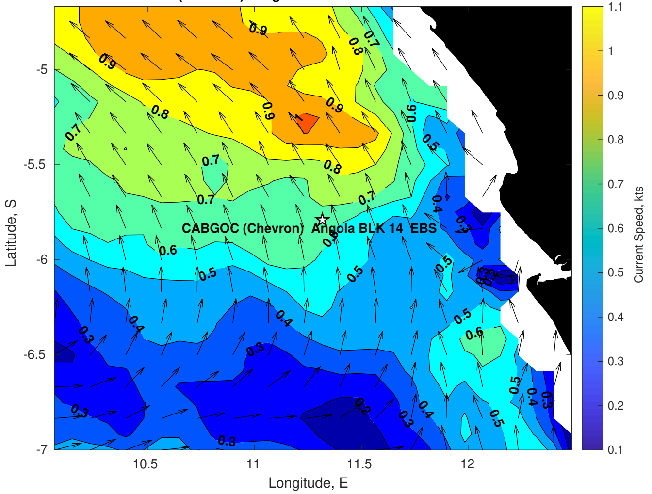
Surface Currents for CABGOC (Chevron) Angola BLK 14 EBS at 11-Feb-2025 00:00:00
