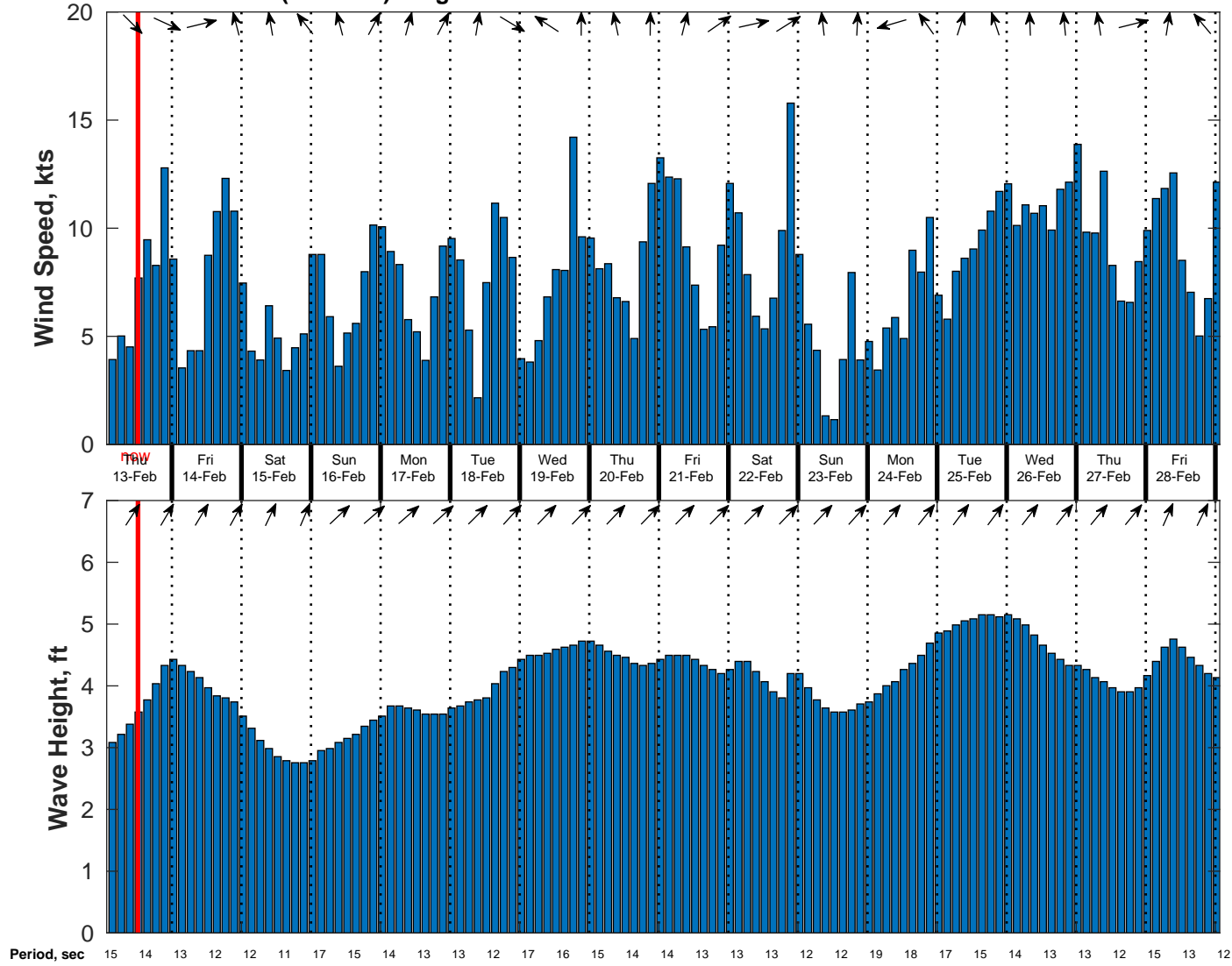
Wind & Wave Forecast for CABGOC (Chevron) Angola BLK 14 EBS from 12-Feb-2025 02:00:00 to 28-Feb-2025 02:00:00
