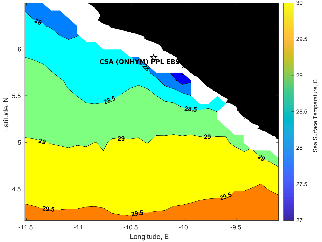
SST for CSA (ONHYM) PPL EBS - Liberia at 11-Feb-2025 00:00:00
