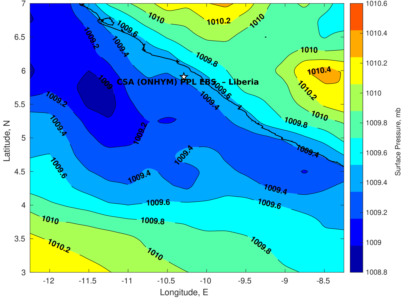
Surface Pressure (mb) for CSA (ONHYM) PPL EBS - Liberia at 12-Feb-2025 00:00:00
